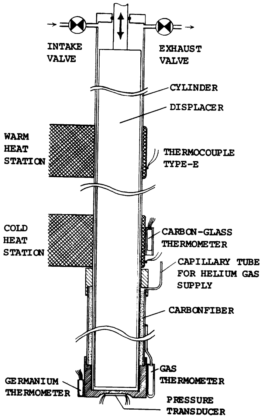
Figure 4. Gap regenerator/expander with pressurized helium gas annulus.
