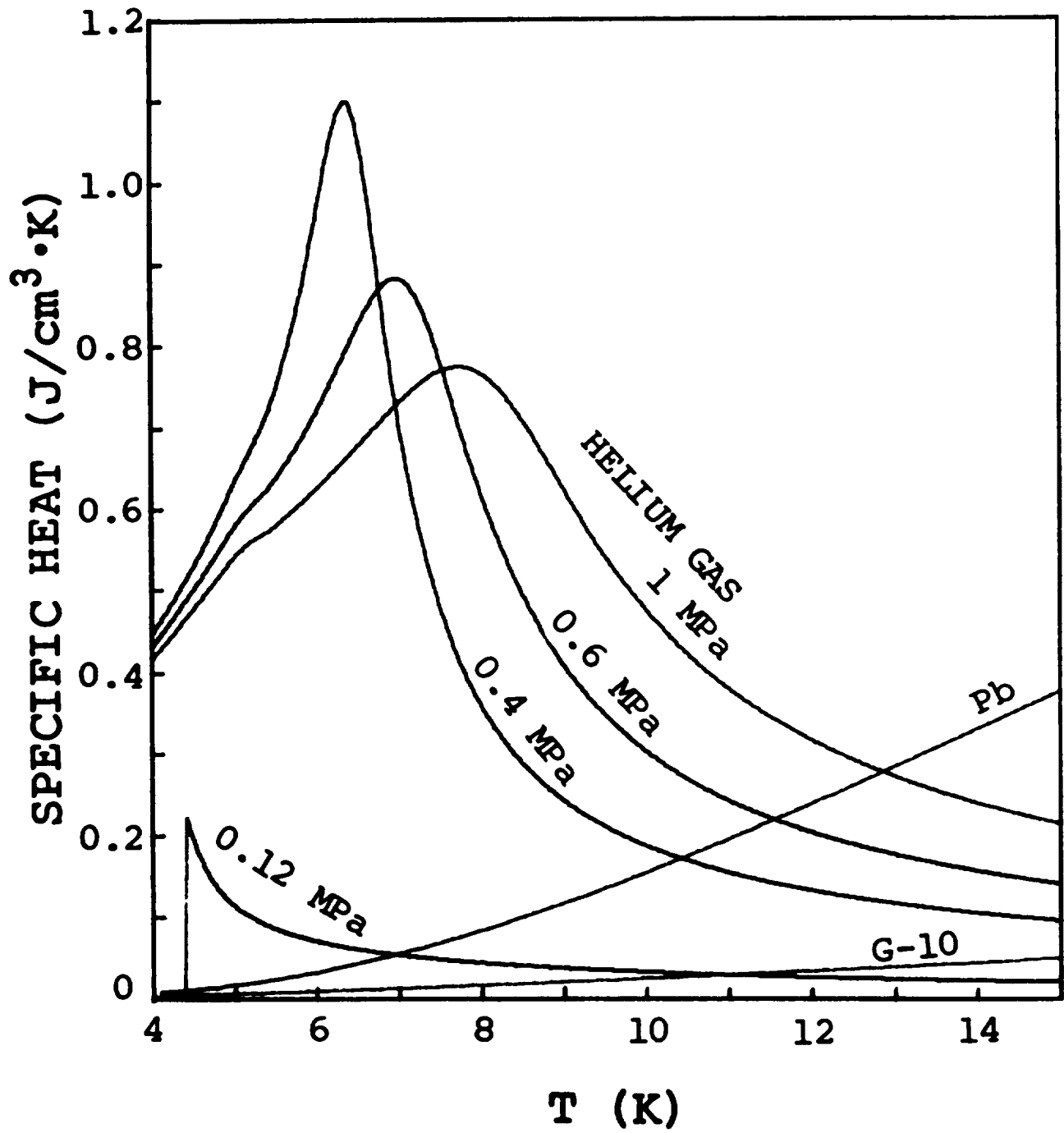
Figure 1. Volumetric heat capacity of helium, lead and G-10.
