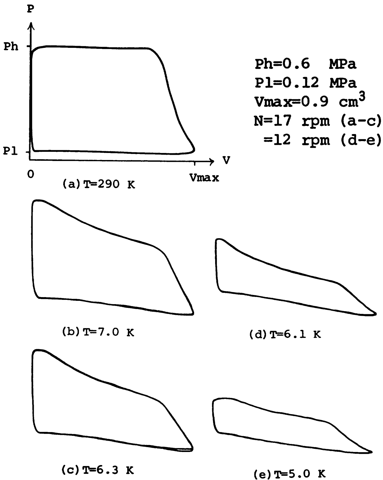
Figure 5. P-V diagrams of the expander.
