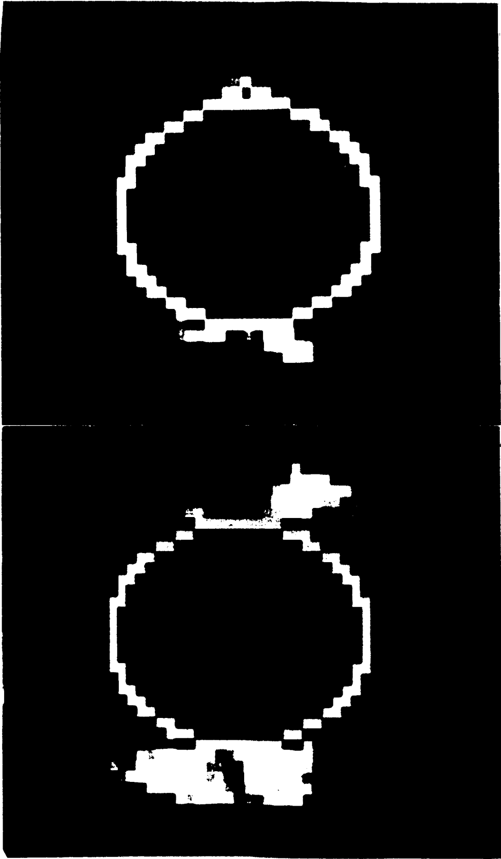
(a) (b) Figure 1. (a) A grey-scale picture of the solar green-line corona from 1.15 to 1.55 R_{\odot} taken from 14:49 to 15:10 UT on 19 Oct 1982. The bright inner circle represents the solar disk. Intensities have been scaled to yield a constant average intensity with height. Solar north is at the top and east is on the left. Note the two active regions on the east limb and one on the west limb. (b) A difference picture of the solar green-line corona, with the scan of (a) subtracted from one made from 22:02 to 22:25 on the same day. The transient discussed in the text is on the left, just below the equator (azimuth angle 105°). Two other transients are visible near azimuth angles 80° and 270°. The intensity scale is not the same as in (a).
