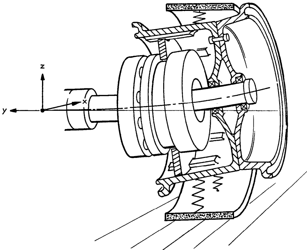
Figure 9.- Brake whirl.
