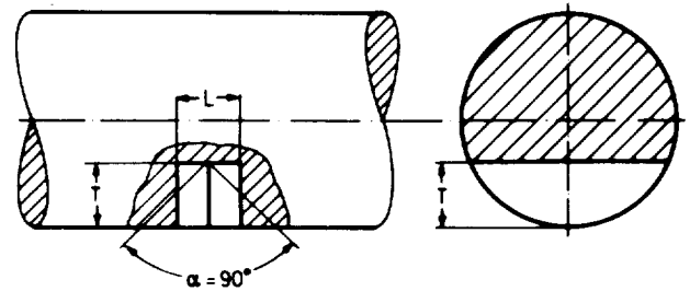
Figure 2. - Simulation of decreased cross-section open crack location.
