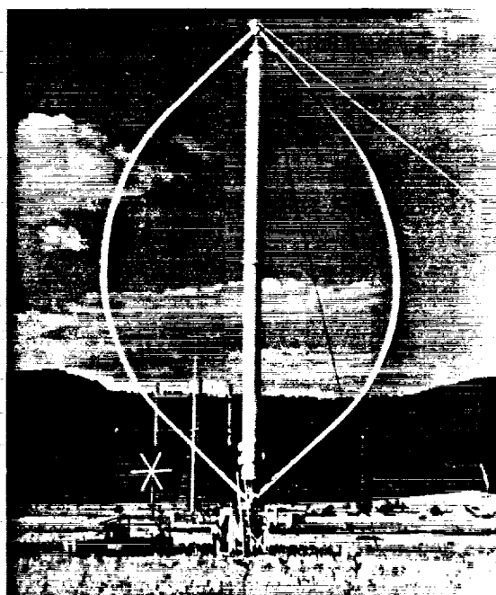
FIGURE 1. DOE/ALCOA Low Cost 17M VERTICAL AXIS WIND TURBINE INSTALLED AT ROCKY FLATS, CO.
