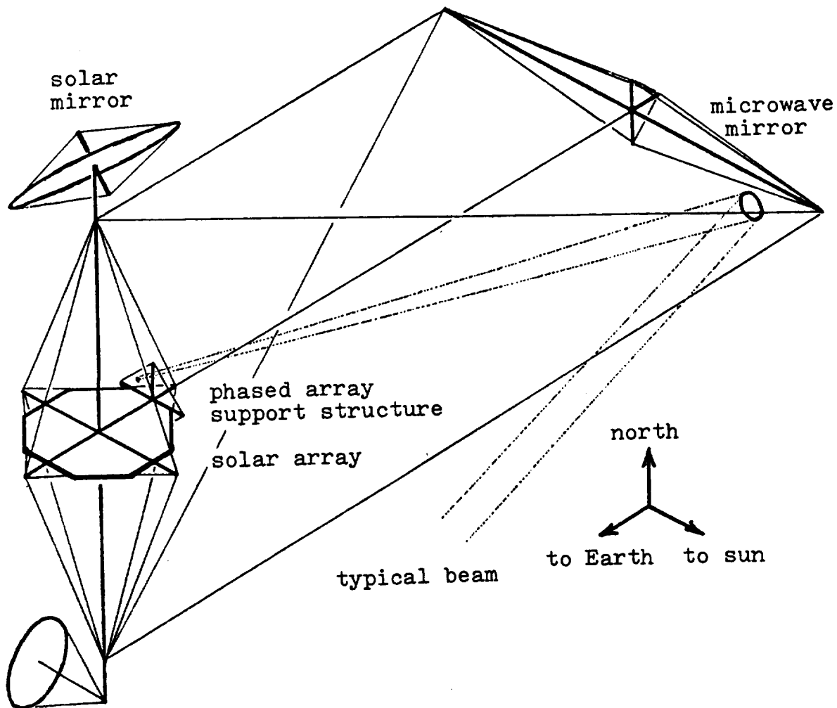
FIGURE 1: A gravity-gradient stabilized configuration, incorporating a rotating solar mirror and no rotating electrical joint. Length about 100 kilometers.
