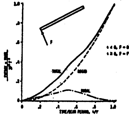
FIGURE 8 - ENERGY IN A BEAM FROM STEP FUNCTION FORCE
