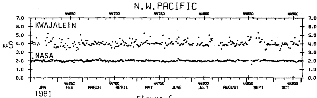
Figure 6. Relative scatter about an offset zero line of Loran-C signals as observed at two separate monitoring sites in the Pacific.
