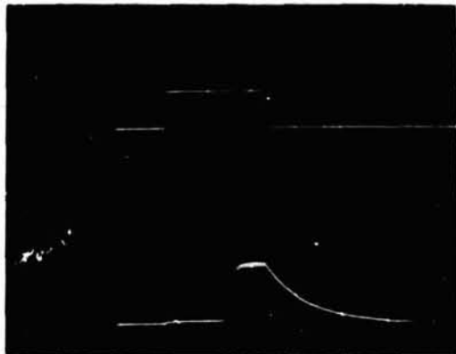
Fig. 5. Scope trace of unstable switching pulses. Cd-Cl boracite sandwich electrode sample with electrode spacing of 0.48mm; voltage (upper trace) of 5V/div; current (lower trace) of 40 \mu A/div; time of 5 \mu sec/div; pulse repetition rate of 2 KPPS; and temp of 345^\circ \pm 2^\circ\text{C} .
