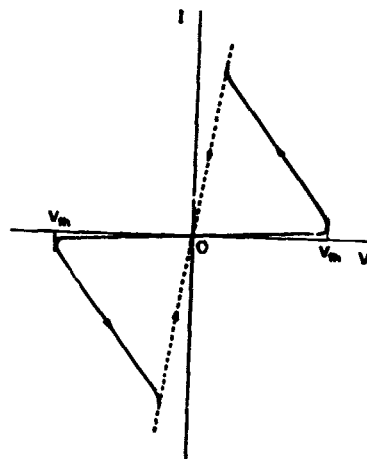
Fig. 1. dc current-voltage characteristics of a Cd-X boracite crystal ( X = Cl or Br) at T \geq T_c .
