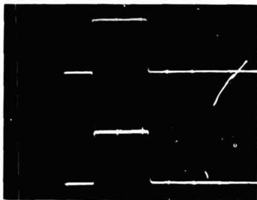
Fig. 6. Scope trace of stable switching pulses. The sample is the same as in Fig.5 with voltage (upper trace) of 2V/div; current (lower trace) of 40 \mu A/div; time of 5 \mu sec/div; pulse repetition rate of 10 KPPS; and temp of 345^\circ \pm 2^\circ\text{C} .
