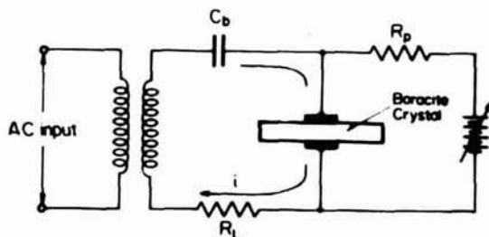
Fig. 7. Circuit of half-wave boracite rectifier.
