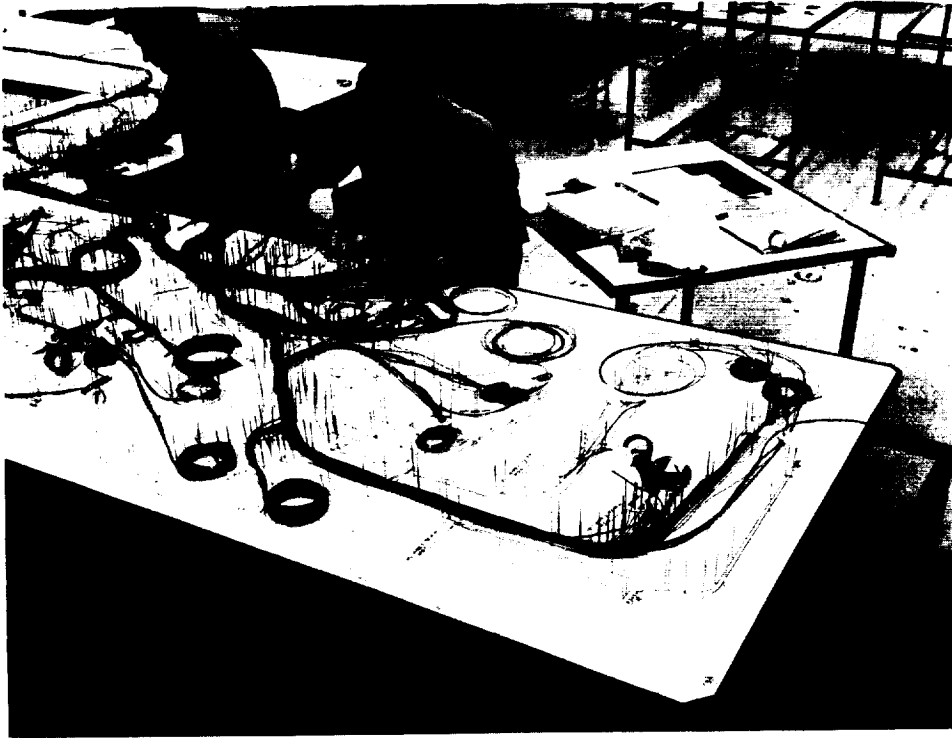
North American manufacturing personnel route electrical wires on a jig board as they prepare the CM 107 crew compartment wiring harness.
