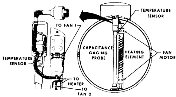
Apollo 13's service module oxygen tank, left. Redesigned oxygen tank below.
