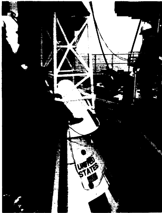
The launch escape system is mated to Apollo spacecraft 009 atop the Launch Complex 34 service tower at Cape Canaveral, in December 1965 preparations for the February 26, 1966, AS-201 mission.
