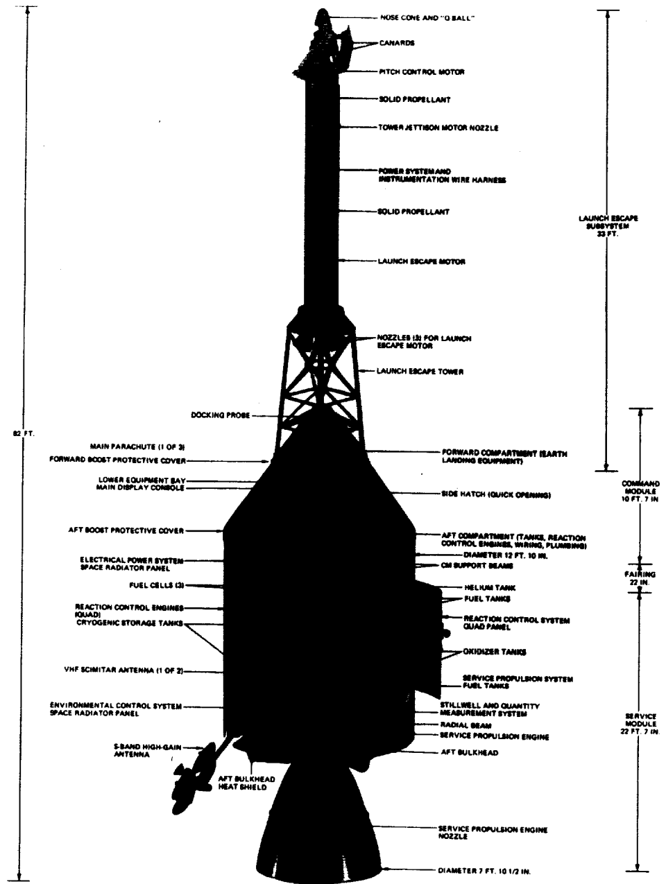
A cutaway view of the Block II CSM configuration and launch escape system shows some of the components.
