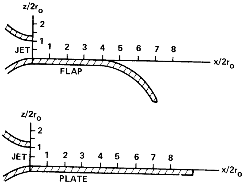
(a) Flow configurations.
