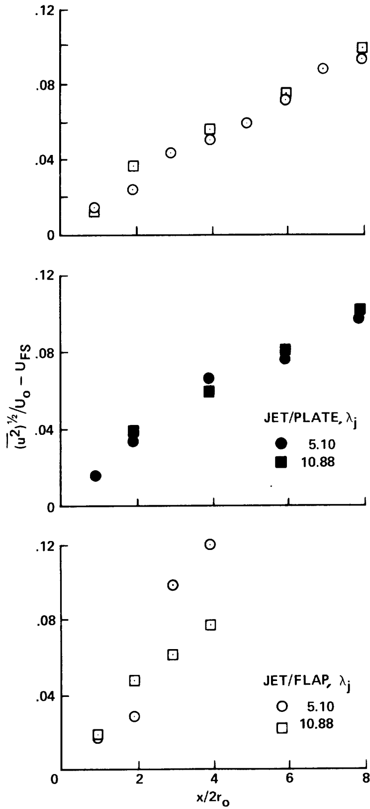
Figure 5.- Growth of turbulent intensity, (\overline{u^2})^{1/2} , at centerline.
