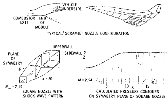
Figure 6. Integrated Scramjet Nozzle
