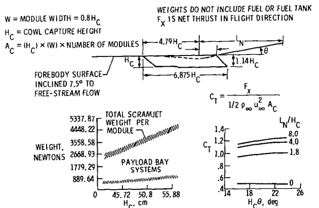
Figure 14. Scramjet Weight and Nozzle Geometry
