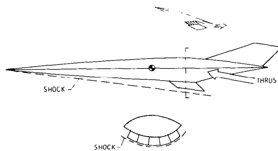
Figure 2. Scramjet-Vehicle Integration
