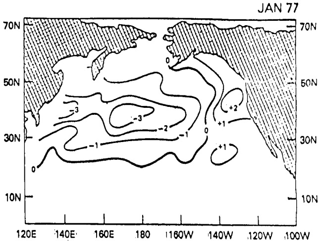
Fig. 1. Observed sea surface temperature anomaly ( ^{\circ} F) during January 1977.
