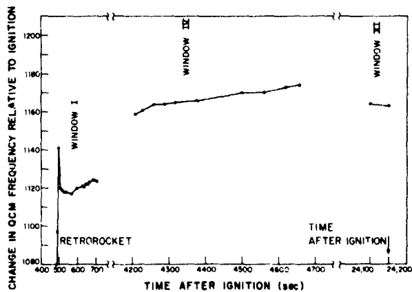
QCM FREQUENCY VS. TIME FOR WINDOW IV, XI, AND END OF I
