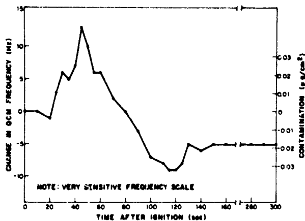
QCM FREQUENCY VS. TIME: IGNITION TO PLF JETTISON FIGURE 6
