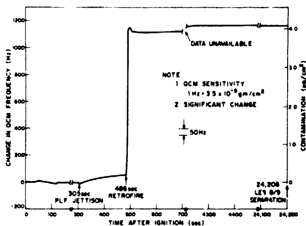
QCM FREQUENCY VS. TIME FOR ENTIRE LAUNCH FIGURE 5
