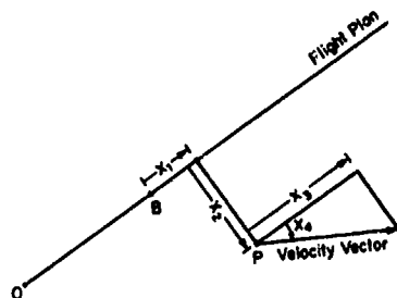
Figure 4. Choice of Co-ordinates for System Equation
