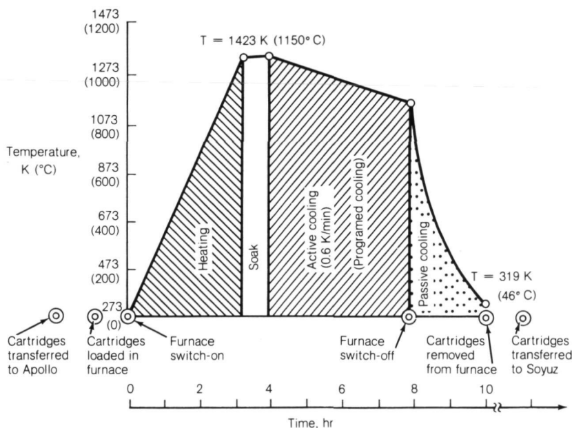
Figure 3.7 Temperature versus time in the Soviet materials melting experiment. The ampoules at the hot end produced an aluminum-tungsten alloy. Other ampoules reached lower soak temperatures and produced germanium crystals and aluminum spheres.
