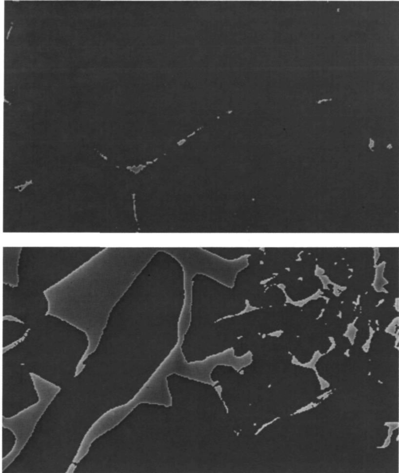
Figure 3.6 Microstructure of AISb formed in zero-g and one-g. These enlarged photographs of polished cross sections of the AISb ingots cooled in zero-g (top) and one-g (bottom) have been colored red for pure AISb and blue for mixed structures. The defective (blue) areas total 1 percent of the area shown in the top photograph and 25 percent of the area shown in the bottom photograph.
