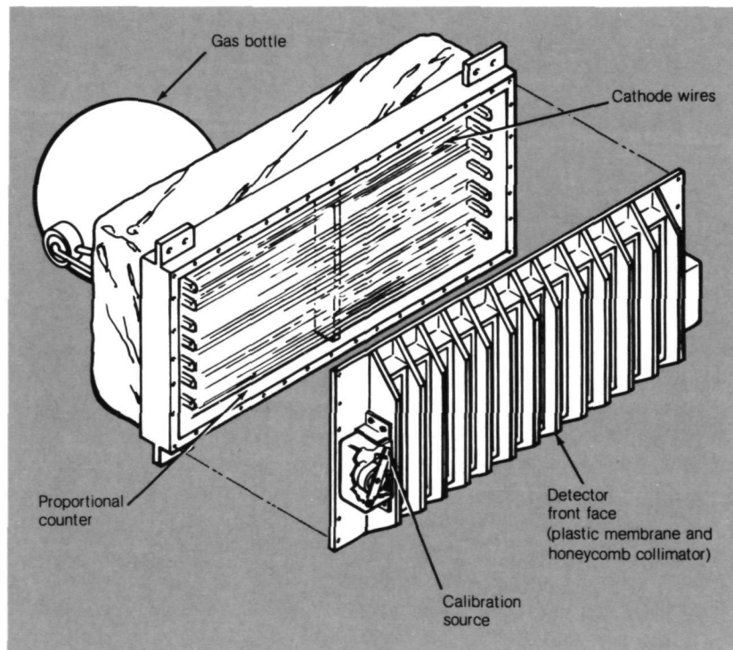
Figure 4.1 The MA-048 soft x-ray detector. The structure of the detector front acts as a collimator.
