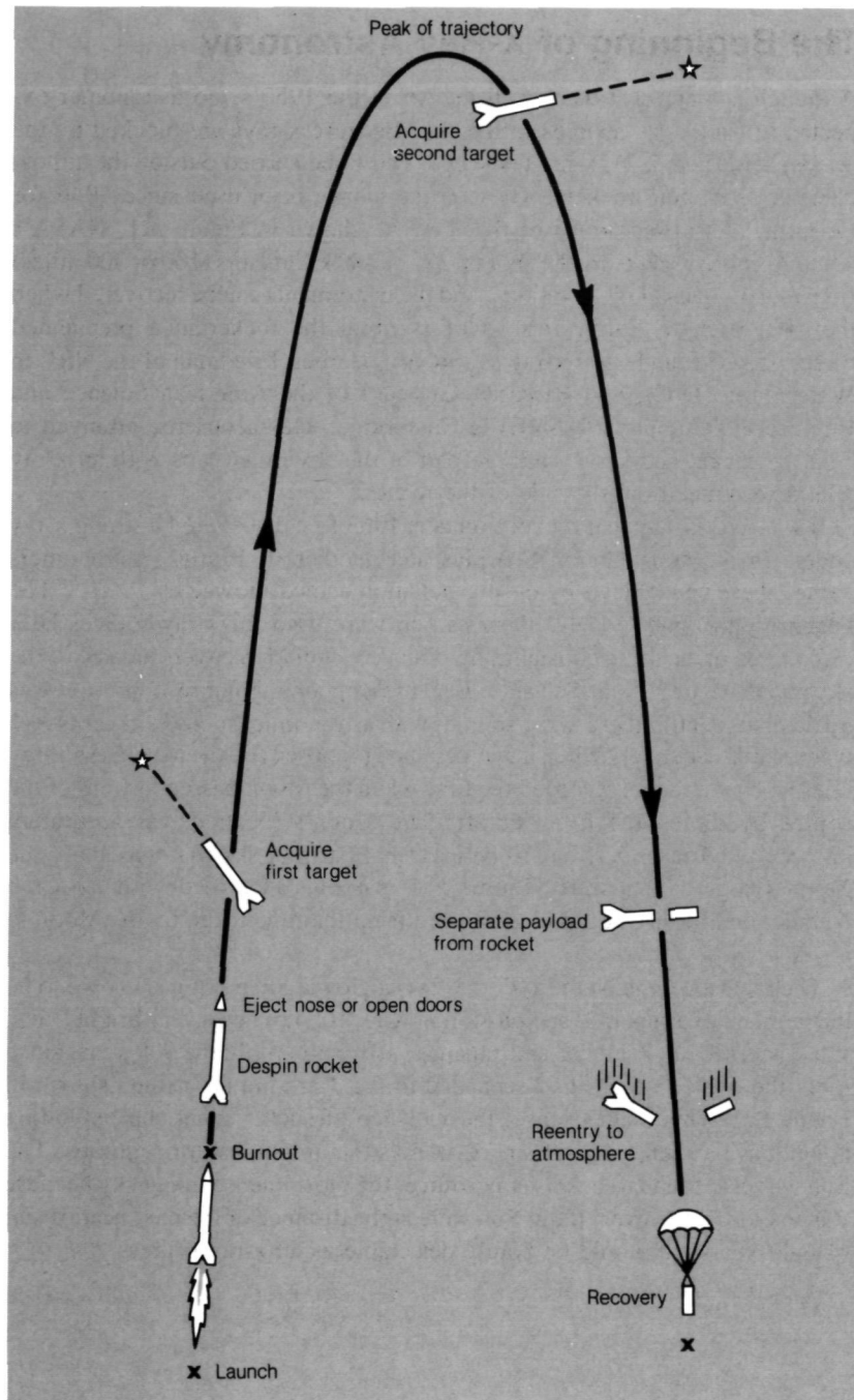
Figure 3.1 Diagram of an Aerobee rocket flight.
