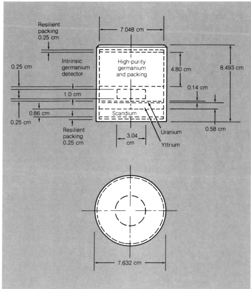
Figure 5.2 Diagram of the MA-151 container holding the germanium crystals and metals.
