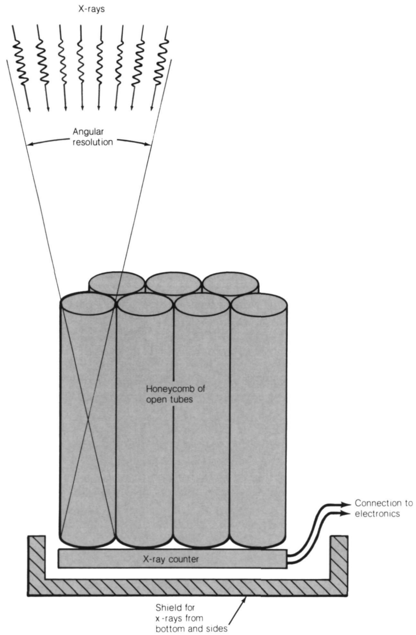
Figure 2.6 X-ray collimator and its angular resolution.
