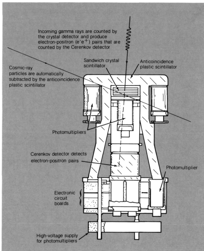
Crystal scintillator gamma-ray detector with anticoincidence counter Figure 2.9 (schematic diagram of one carried on the Explorer 11 spacecraft).
