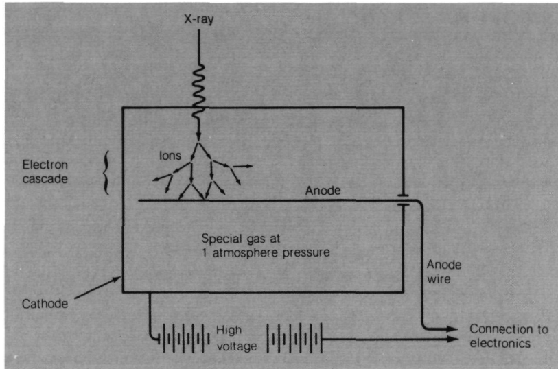
Proportional counter. An x-ray photon ionizes a gas atom, releasing one or more electrons that are accelerated toward the high-potential anode, ionizing more atoms and releasing more electrons—most of them close to the anode. The large electric pulse of this cascade is proportional to the number of ions formed by the x-ray and therefore to the energy of the x-ray photon.
