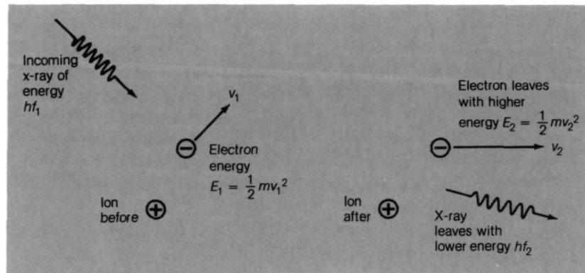
Figure 3.9 The Compton effect. In this interaction between an x-ray and an electron near a positive ion, energy and momentum are conserved.
