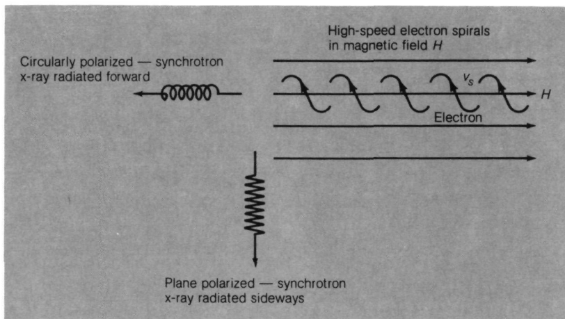
Synchrotron radiation from free electrons moving in a magnetic field H . The field forces the electrons to “spiral” around lines of force. Figure 3.8
