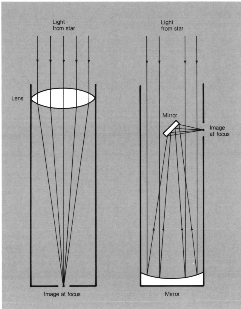
(a) Refractor (lens) telescope.
