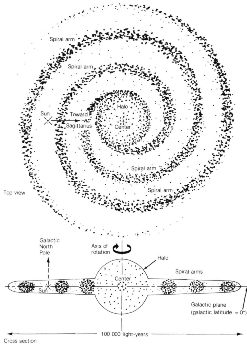
Figure 3.6 Top view and cross section of the Milky Way Galaxy, a gigantic rotating disk of stars, gas, and dust, about 100 000 light-years in diameter and 5000 light-years thick, with a bulge or halo around the center of mass.
