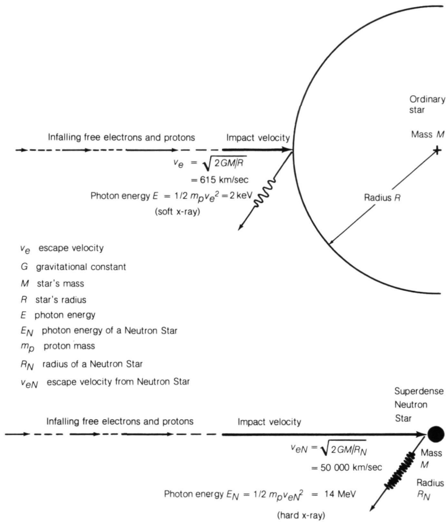
Figure 3.7 Impacts of infalling electrons on stars. Only very dense stars have enough gravitational potential to generate hard x-rays by impact (bremsstrahlung).
