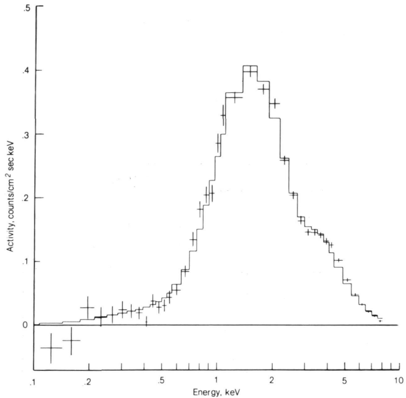
Figure 4.4 Spectrum of Cygnus X-2 observed by the MA-048 Soft X-Ray Experiment.
