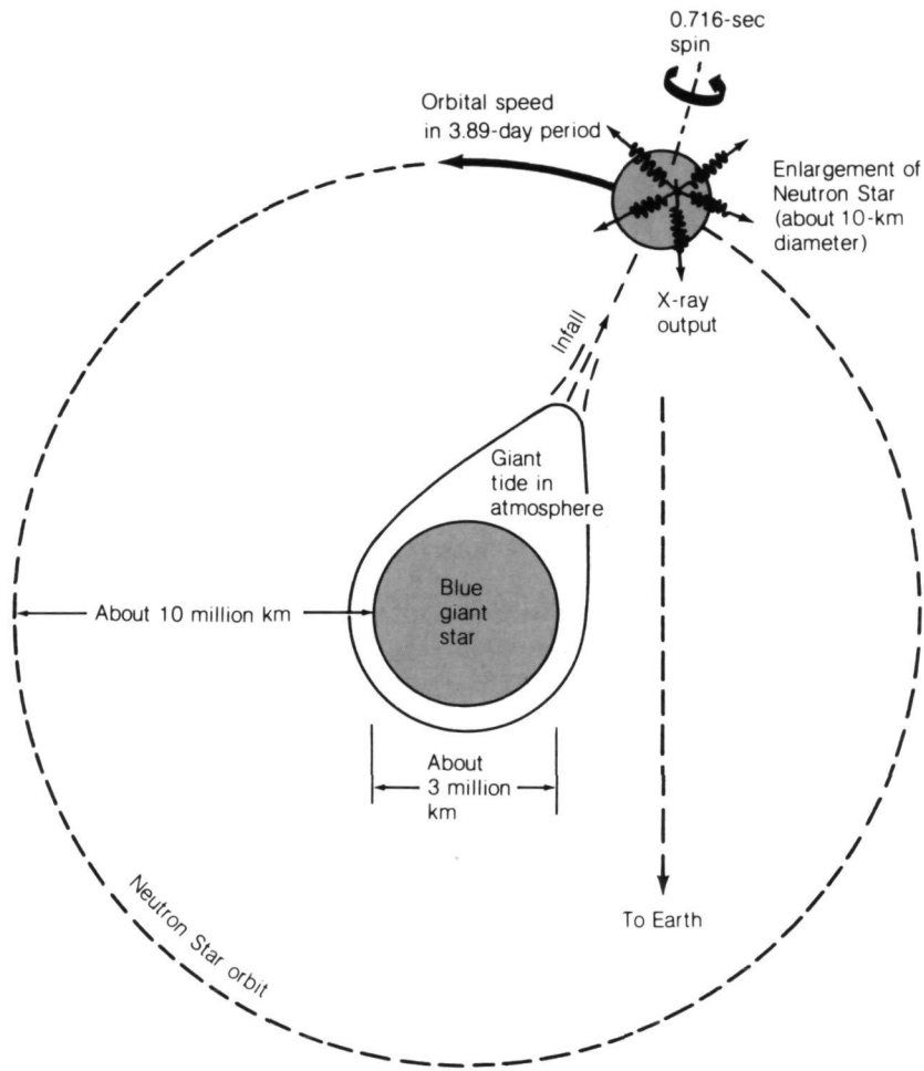
Explanation of the SMC X-1 x-ray pulsar. Figure 4.6
