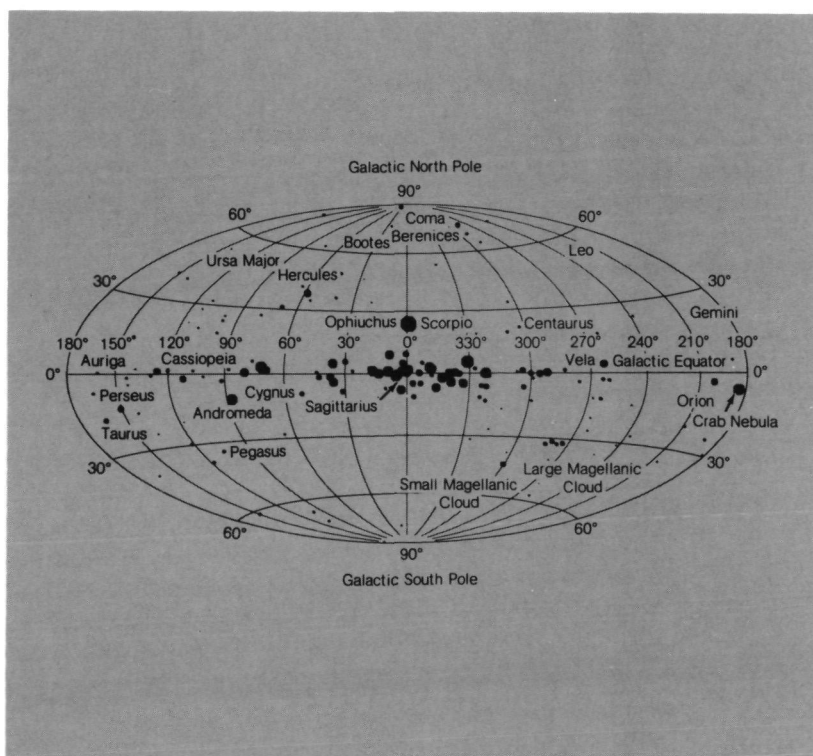
A map of 2- to 10-kiloelectronvolt x-ray sources located in the sky by the Uhuru satellite. Constellation names indicate their approximate areas. Ursa Major is the “Big Dipper.” Sagittarius is in the direction of the center of our Milky Way Galaxy. The Magellanic Clouds are outside galaxies.
