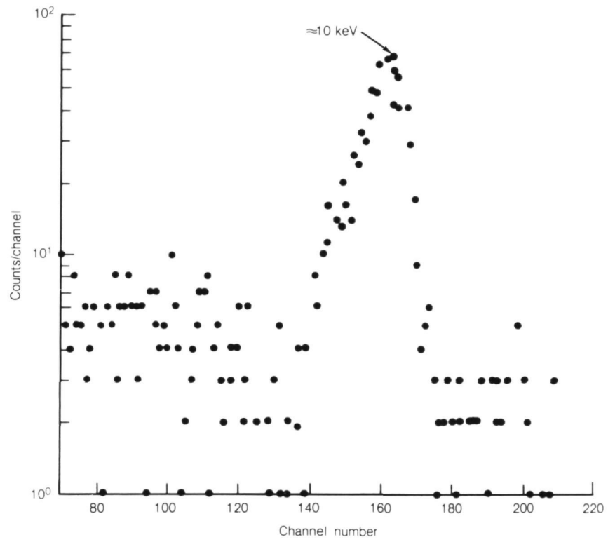
Figure 5.4 Graph of postflight counts in the germanium crystal showing the 10-kiloelectronvolt peak contributed by gallium-67 and germanium-71 (440-minute count time at 0.066 keV/channel).
