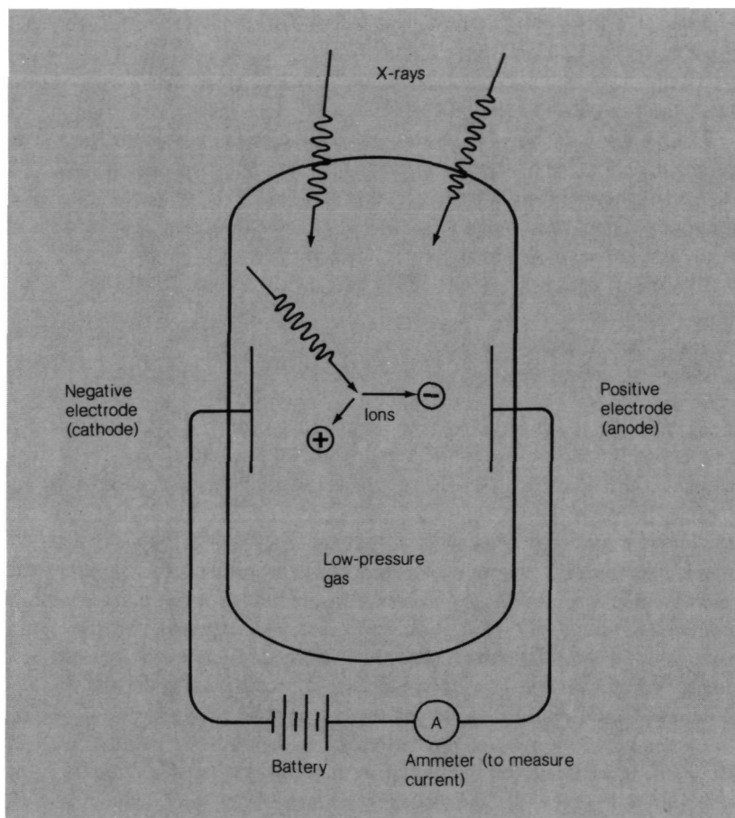
Figure 2.7 Ionization chamber. The current reading at A measures the number of x-rays crossing the tube per second from all directions.
