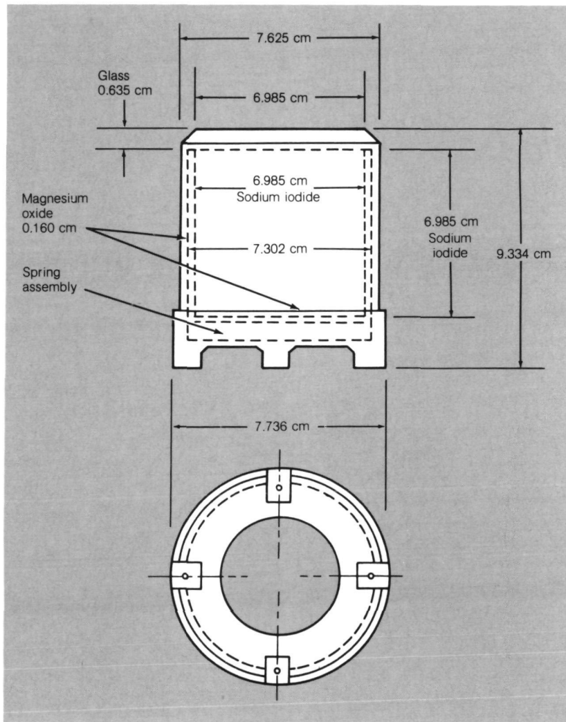
Diagram of the sodium-iodide crystal and cell for the MA-151 Experiment.
