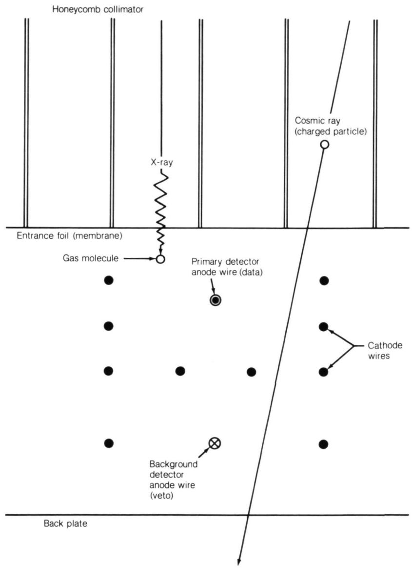
Figure 4.2 Operation of the MA-048 soft x-ray proportional counter.
