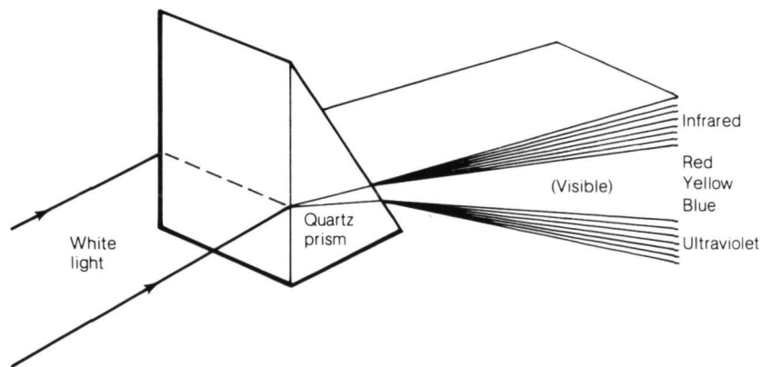
The spectrum of white light. Figure 2.1
