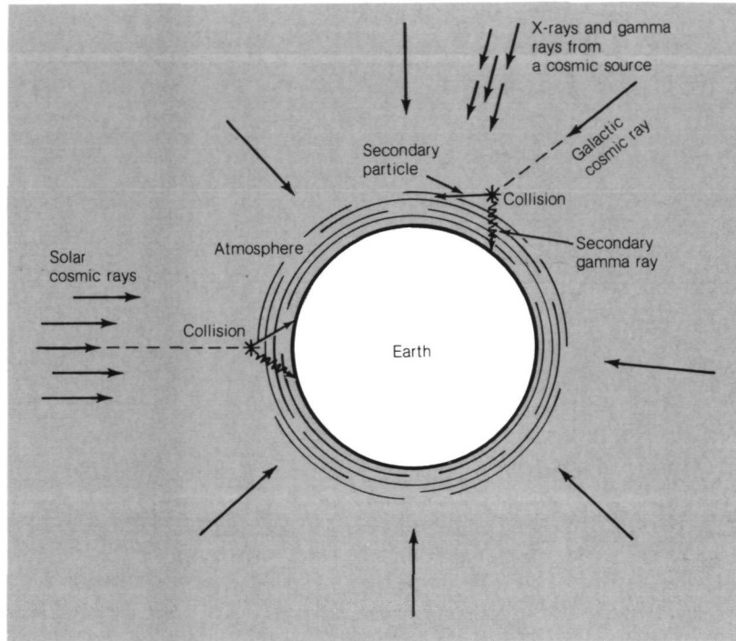
Figure 2.4 High-energy radiation coming in on the Earth.
