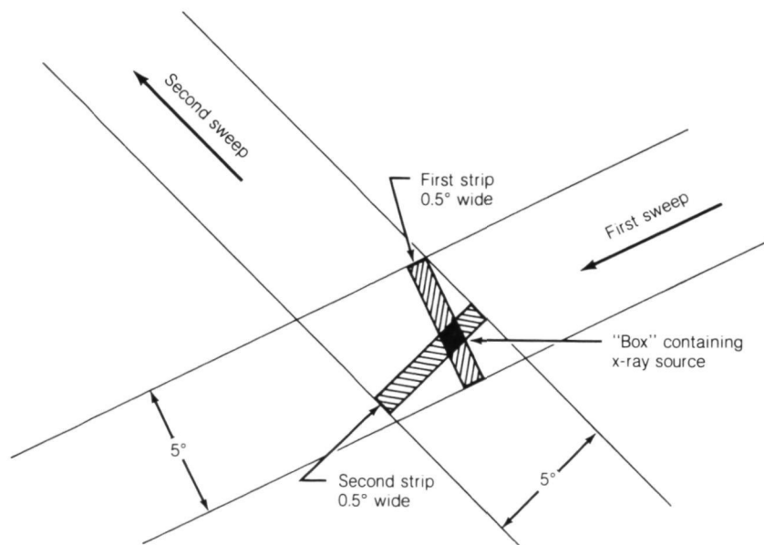
Figure 3.3 Location of an x-ray source in the sky by the Uhuru satellite. Two of Uhuru 's 5° sweeps gave maximum count rates for the heavily outlined strips. The x-ray source must be in the shaded "box" where the two strips cross.
