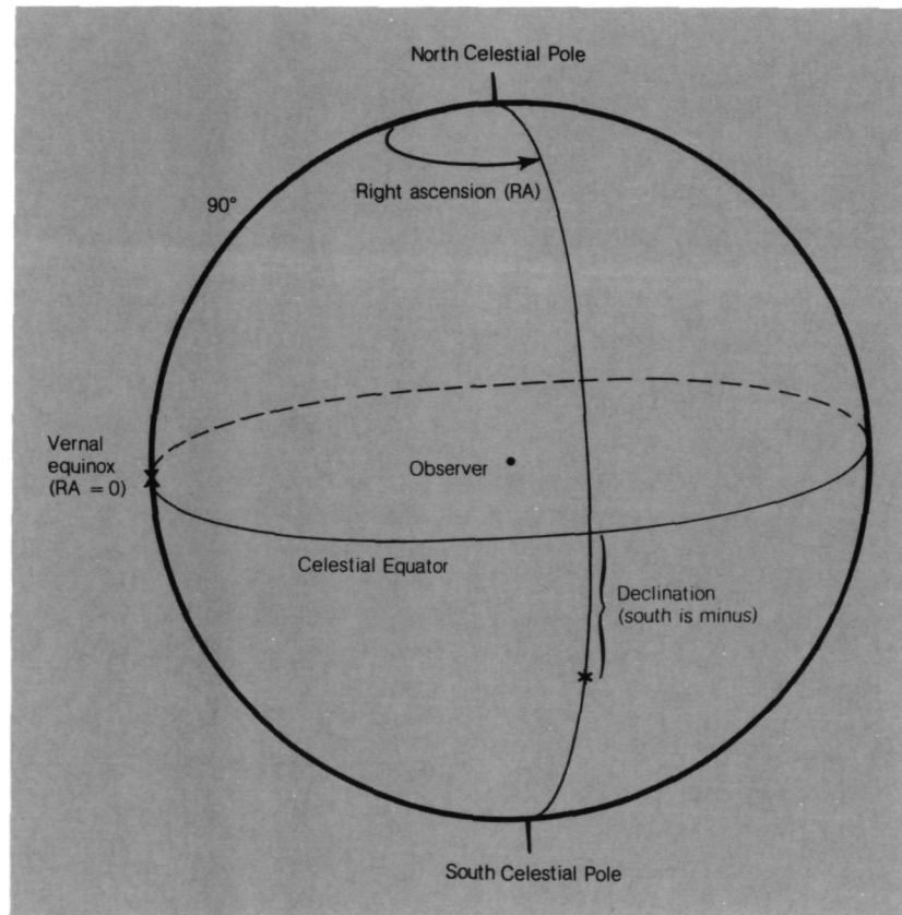
Figure 3.4 Celestial coordinates. The observer is looking outward from the center of an imaginary sphere. Each point in the sky (on the celestial sphere) has its own coordinates, right ascension and declination.
