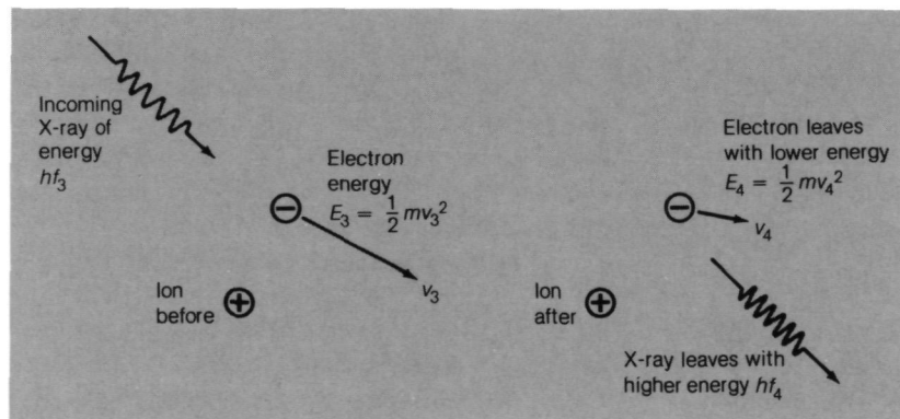
Figure 3.10 The inverse Compton effect. When the angle between an incoming photon and the electron velocity v_3 is correct, the electron loses energy to the photon.
