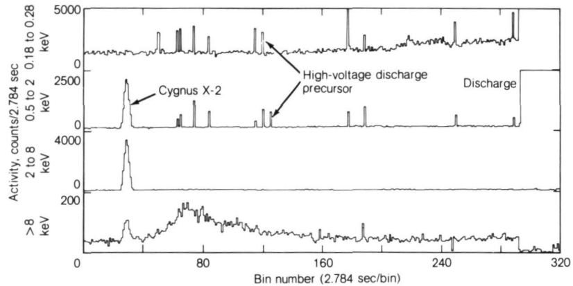
Figure 4.5 MA-048 soft x-ray count rates as a function of time for 14 minutes 51 seconds during the flight, in four energy bands.
