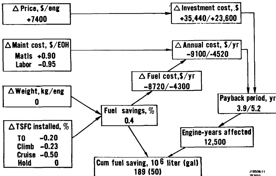
Figure 4.- Evaluation of JT8D revised HPT outer air seal for new buy 727-200/DC9-50.
