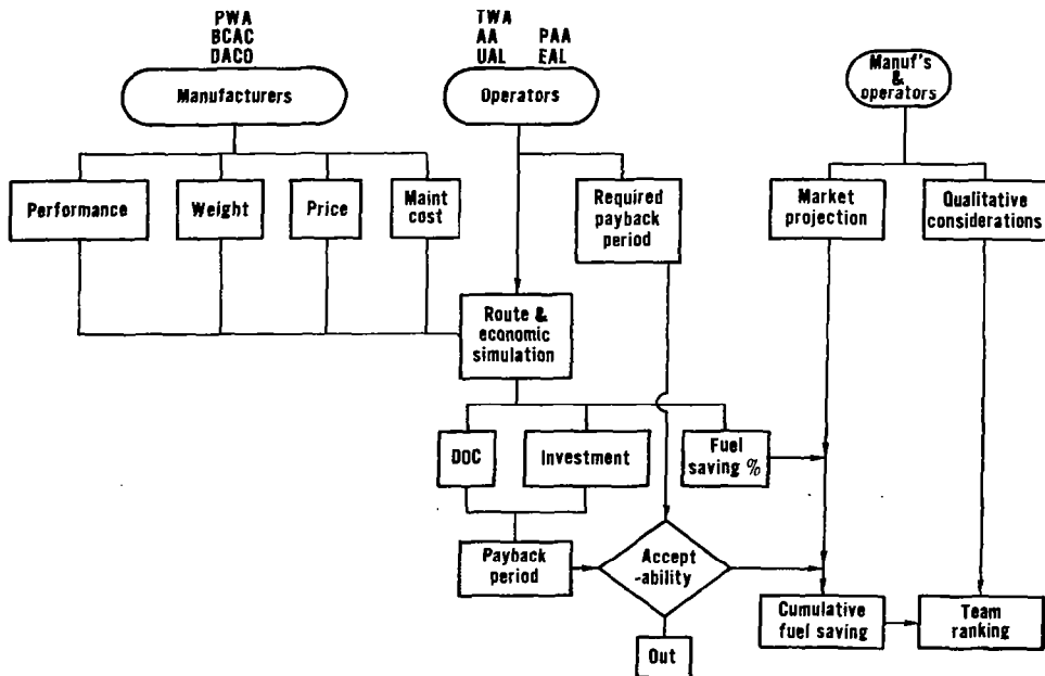
Figure 2.- Detailed evaluation procedure flow chart.
