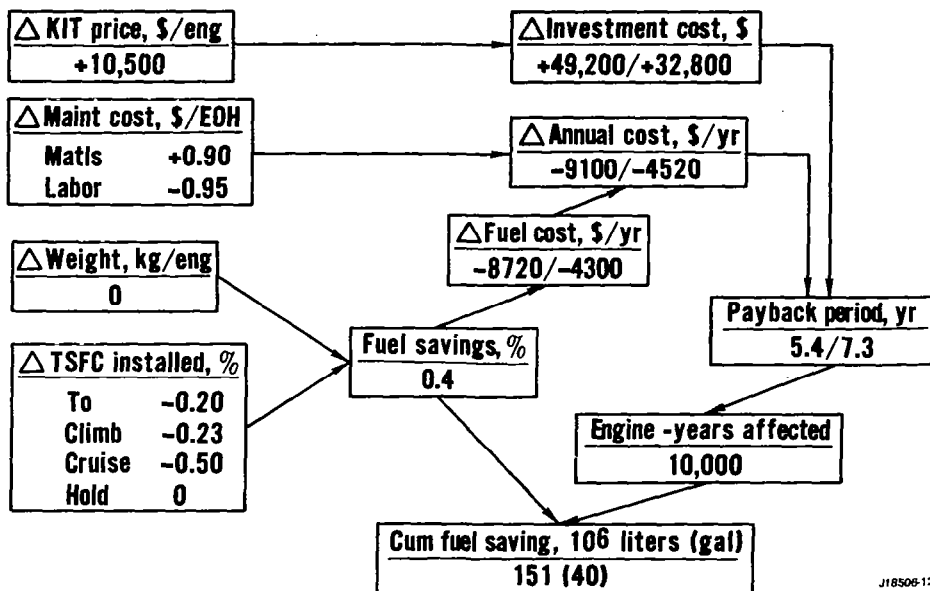
Figure 5.- Evaluation of JT8D revised HPT outer air seal for retrofit 727-200/DC9-50.
