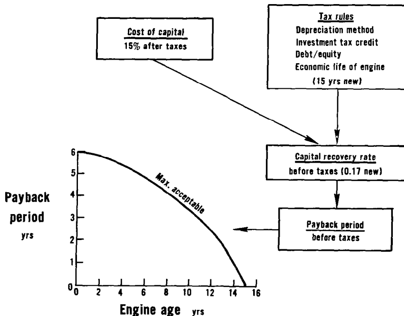
Figure 6.- Maximum acceptable payback period determination.
