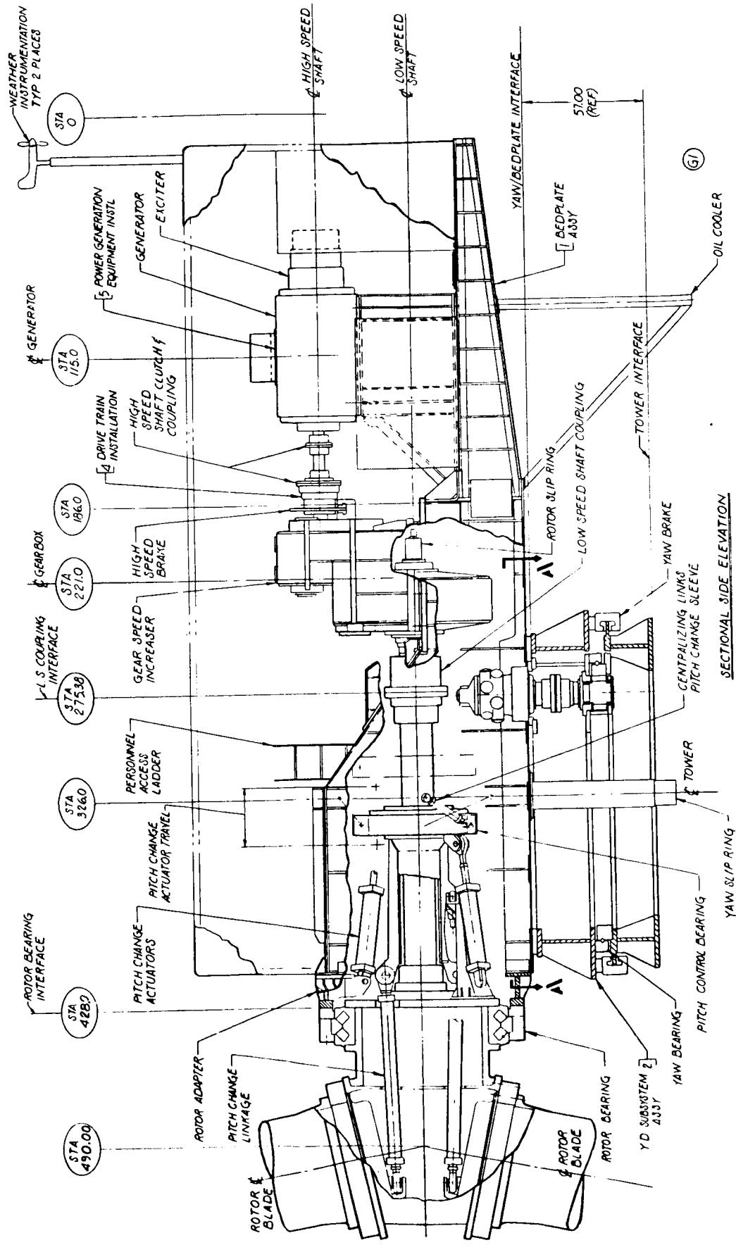
Figure 3. - Nacelle installations.
