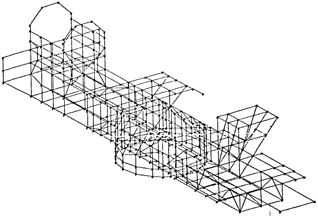
Figure 9. - NASTRAN model of MOD-0 bedplate.
