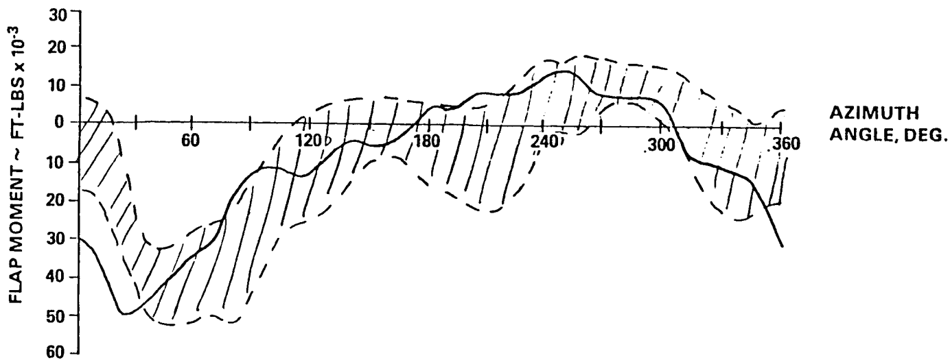
Figure 10. - Case 4 blade load comparison, flap moment at station 40.
