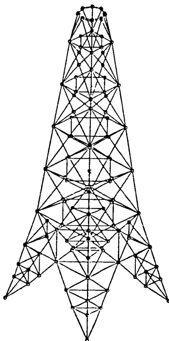
Figure 11. - Finite element model of MOD-0 tower.
