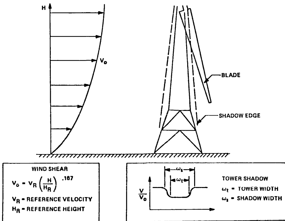
Figure 7. - Wind shear and tower shadow representation.
