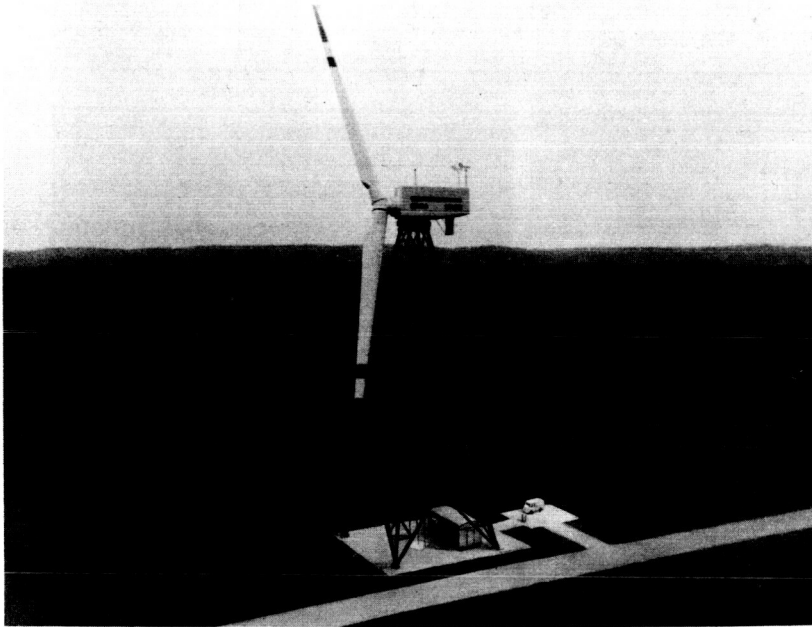
Figure 1. - MOD-1 wind turbine generator.
