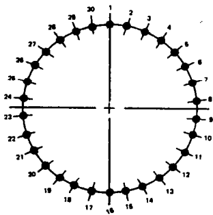
PILOT ZONE FUEL NOZZLE NUMBER LOCATIONS (REAR VIEW SCHEMATIC)
