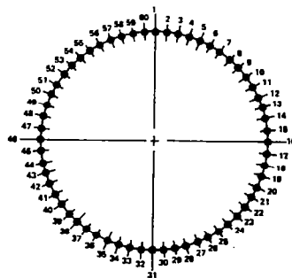
MAIN ZONE FUEL NOZZLE NUMBER LOCATIONS (REAR VIEW SCHEMATIC)
