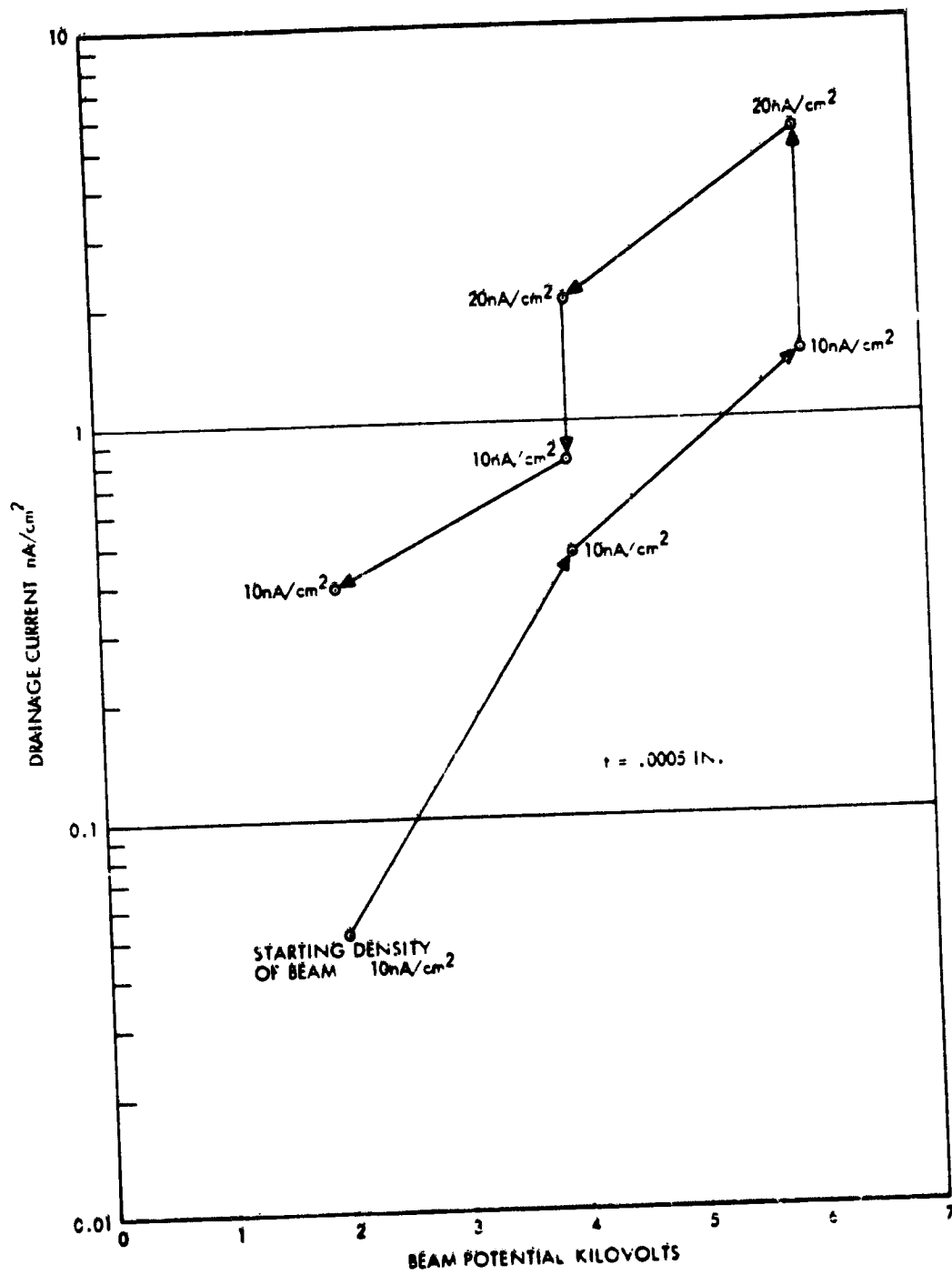
Figure 11. Electron Drainage Current Density as a Function of Electron Beam Acceleration Voltage for Deposition Flux Densities of 10 nA/cm 2 and 20 nA/cm 2 on JRCO Utilizing 0.0005 in. Kapton Base Film
