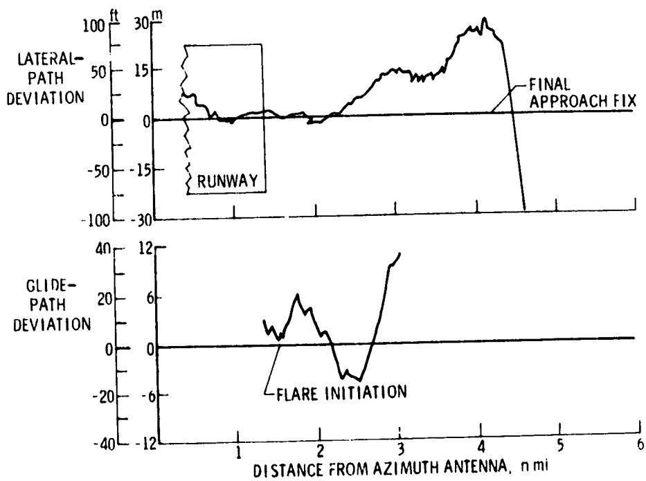
Figure 22.- Typical manual control flight-path deviations.
