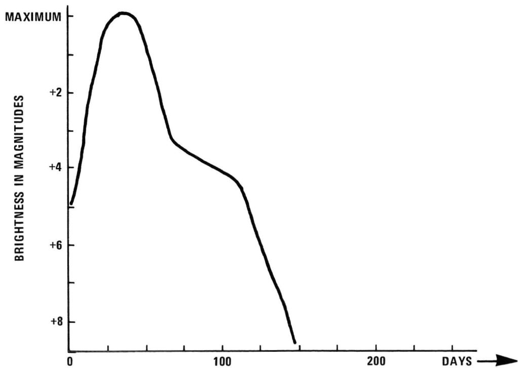
Figure 6. Type II supernova compiled from various sources.
