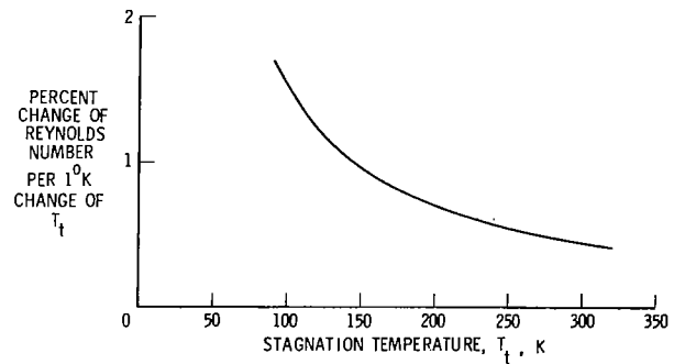
Figure 4. Change in Reynolds number per 1^\circ change in stagnation temperature.
