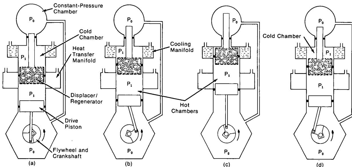
Figure 1. Simplified-Heat-Engine Cycle
