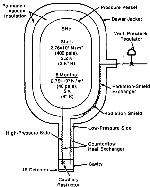
Refrigerator Schematic
