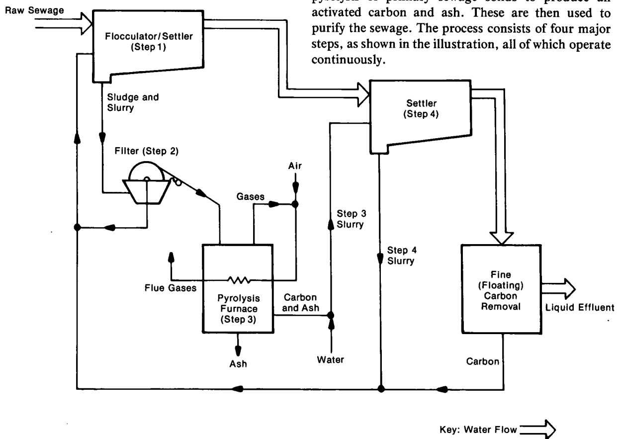
Sewage Treatment Process
