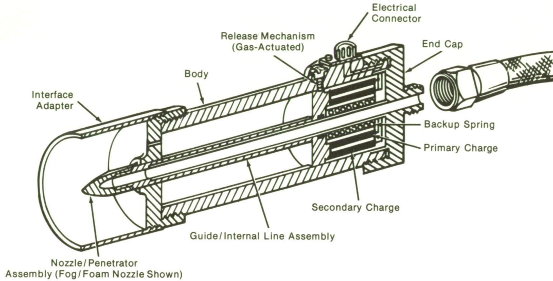
Figure 2. Explosive-Powered Nozzle
