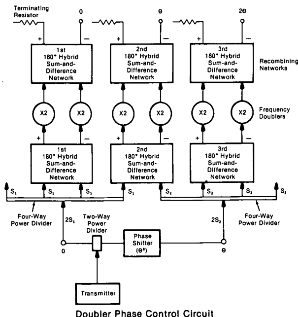
Doublor Phase Control Circuit
