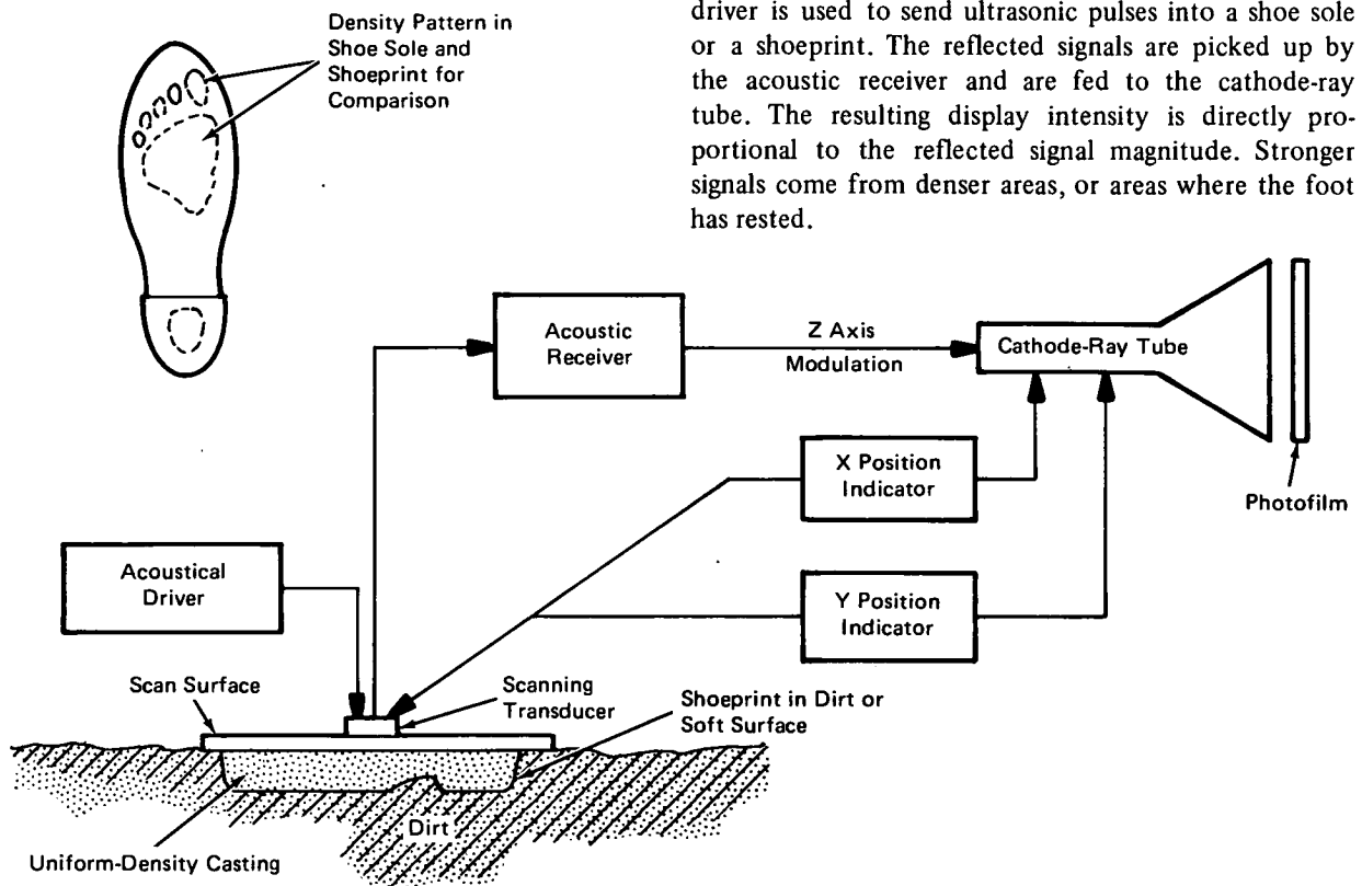
Ultrasonic Scanner System
