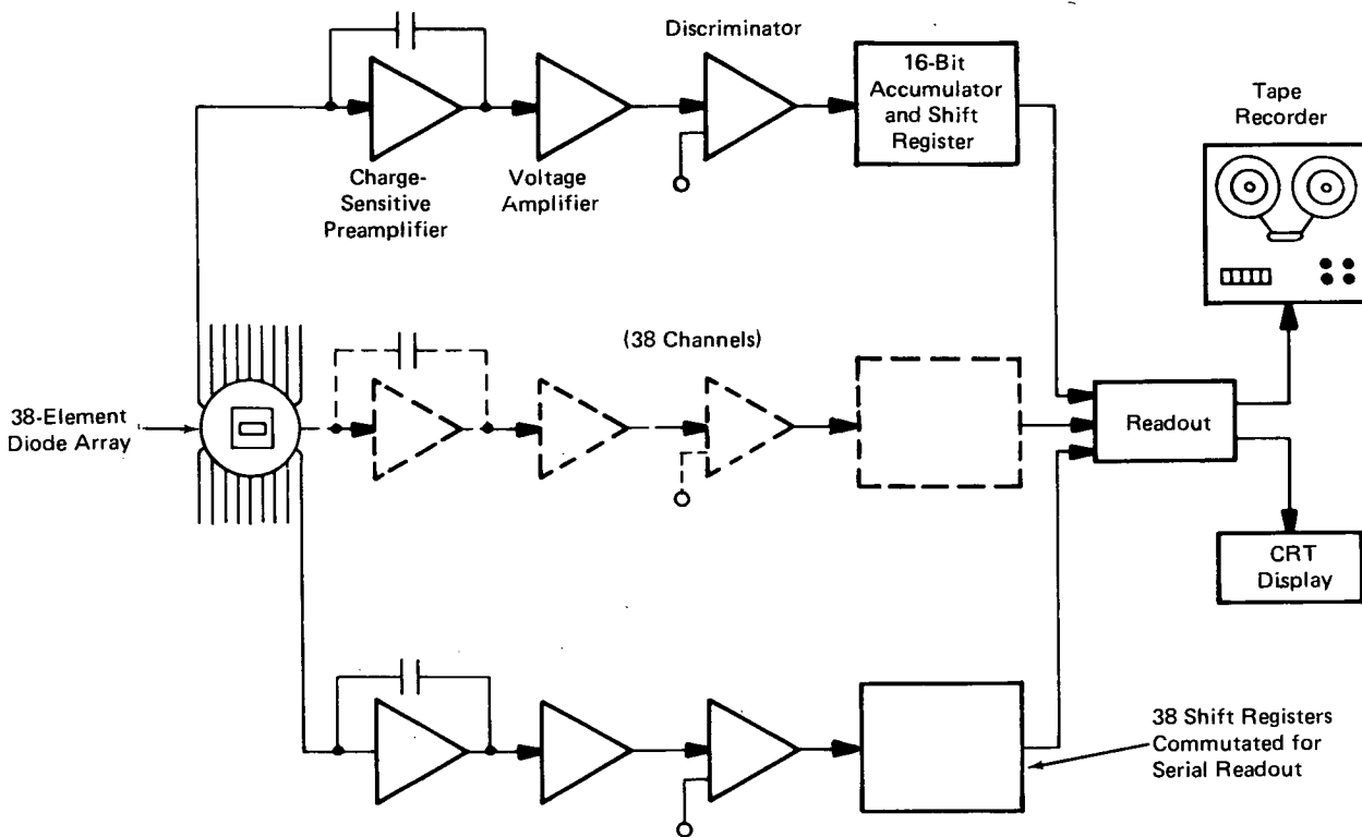
Figure 2. Photometer System
