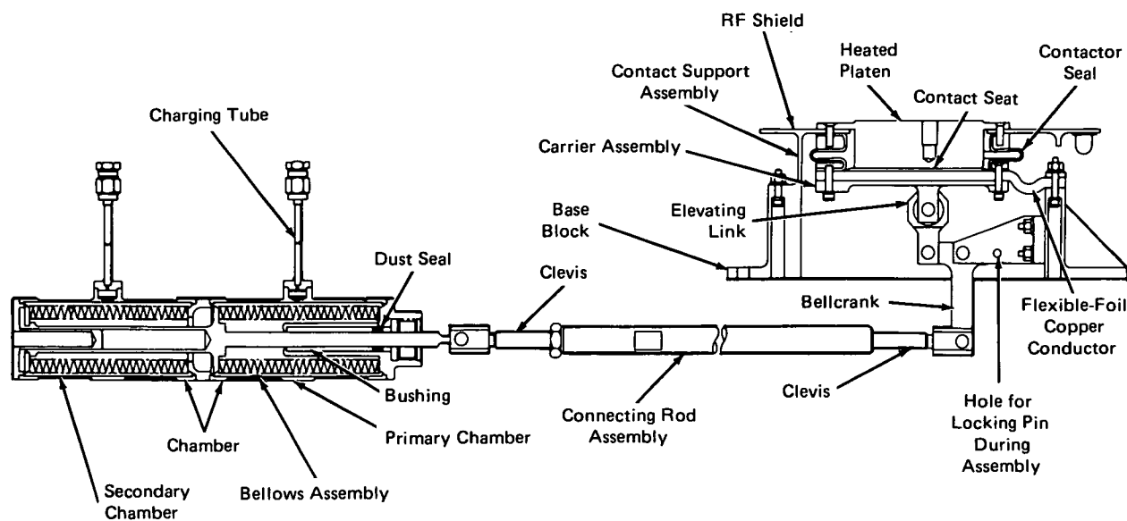
Heat-Transfer Thermal Switch
