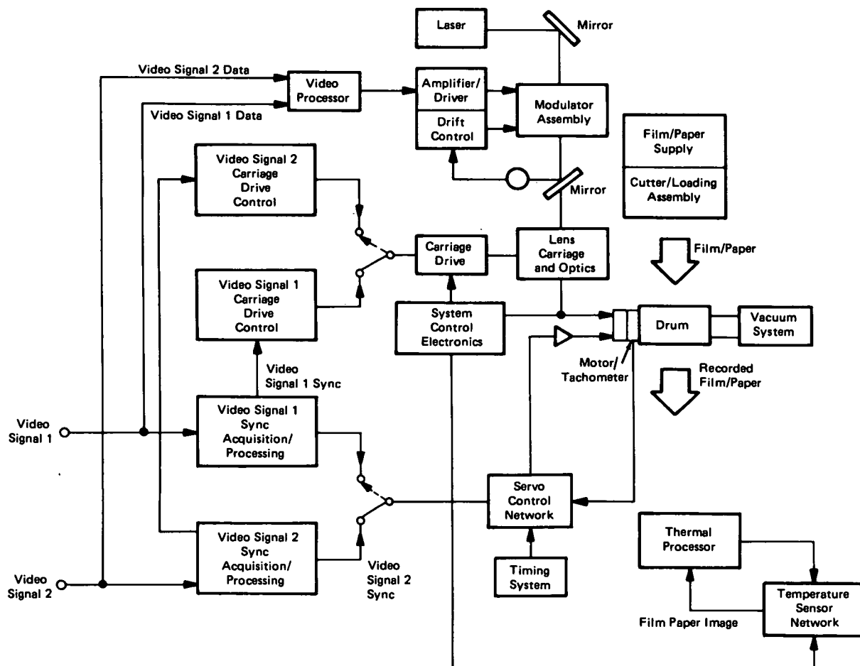
Recorder/Processor Block Diagram
