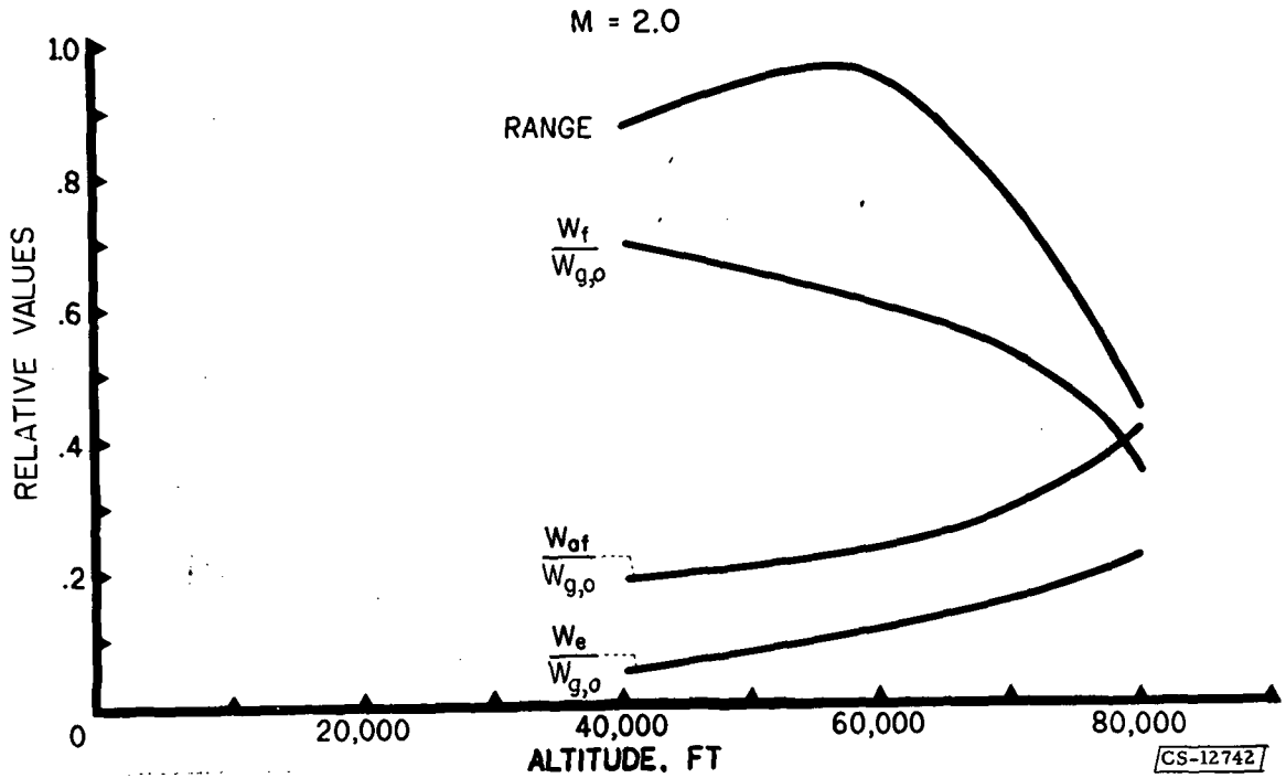
Figure 5. - Relation of altitude to airplane weight distribution.
