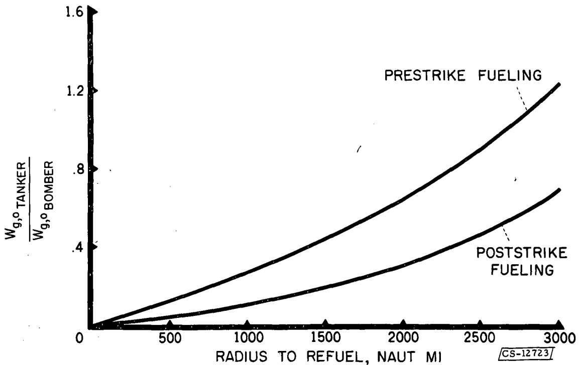
Figure 16. - Relation of tanker weight to bomber weight.
