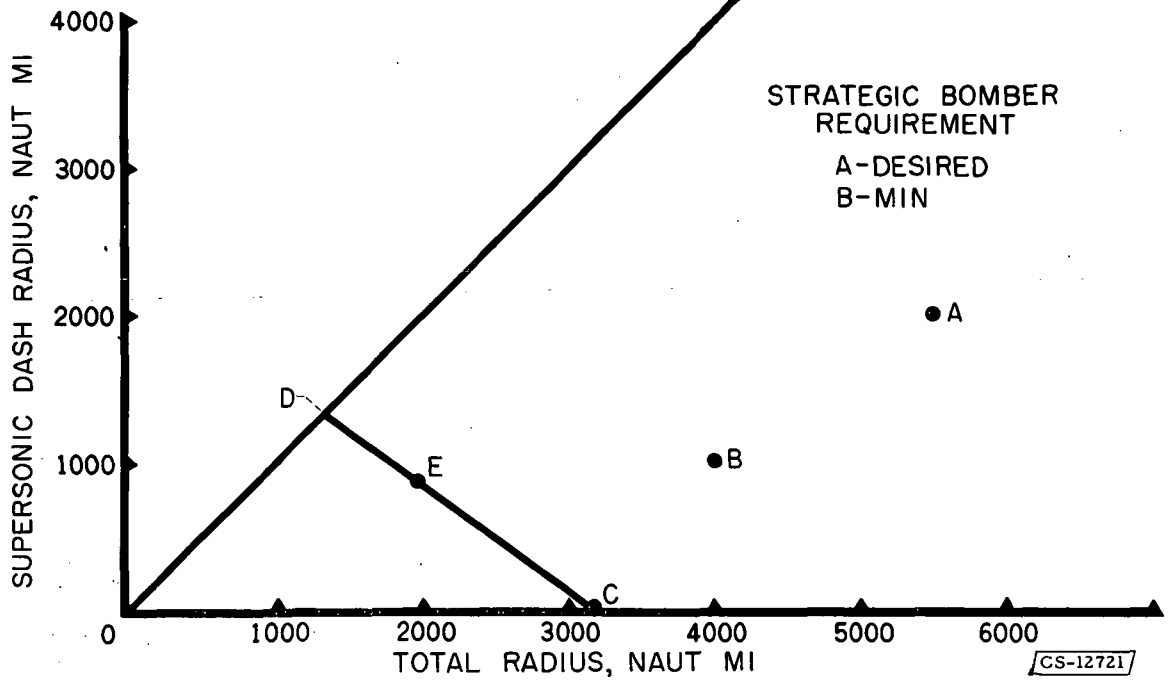
Figure 11. - Supersonic dash vs total radius using JP-4.
