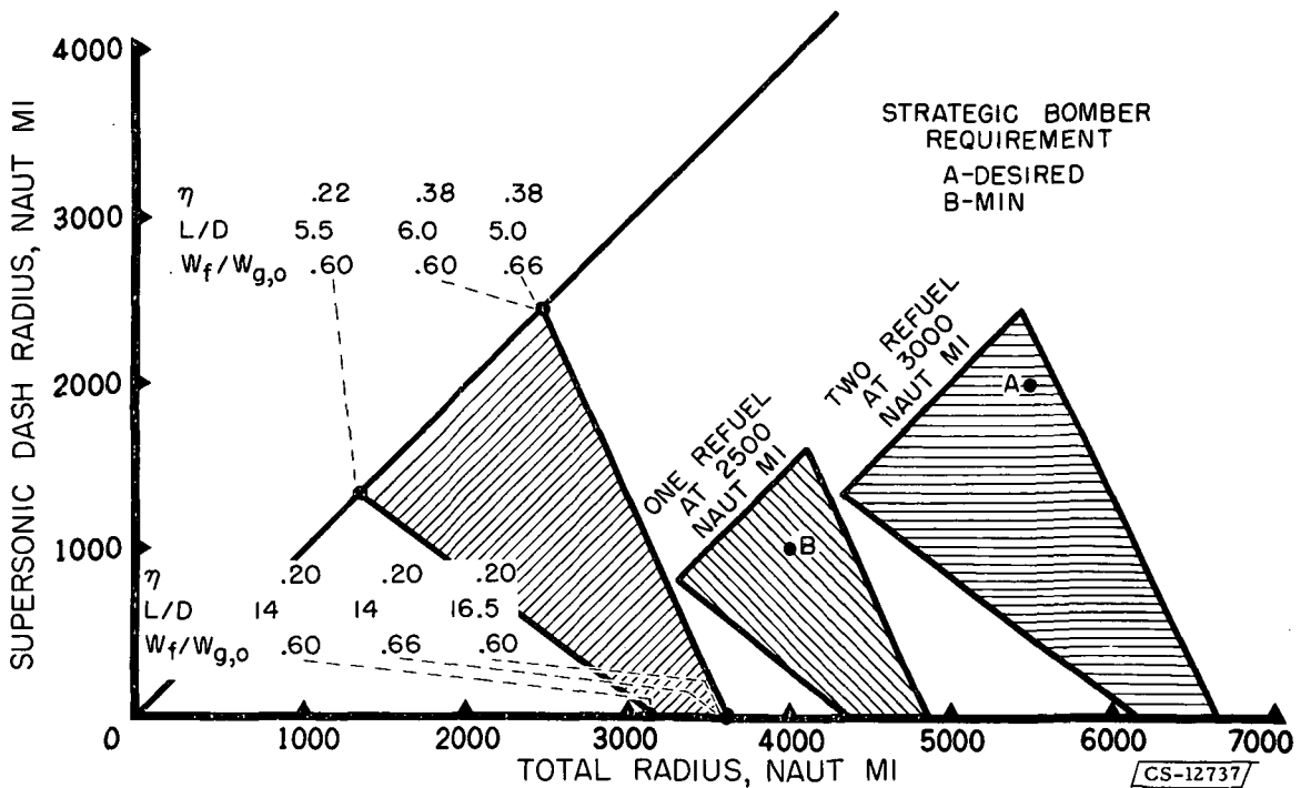
Figure 18. - Supersonic dash vs total radius using JP-4.
