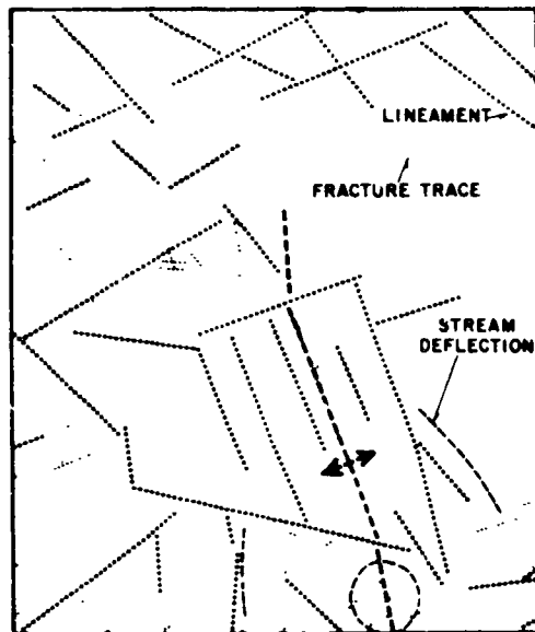
Fig 7 - CENTRAL BASIN PLATFORM, WEST TEXAS ERTS DATA
