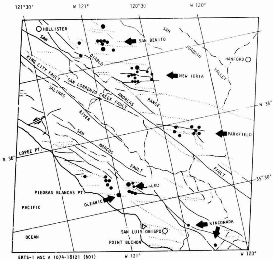
RELATION OF MERCURY DEPOSITS TO TRANSVERSE FAULTS COAST RANGES CALIFORNIA LEGEND — KNOWN FAULTS ..... FAULTS INFERRED FROM ERTS - - - DRAINAGE LINE ← MERCURY MINING DISTRICT ●●● MERCURY MINES Abdel-Gawad & Silverstein 1973
