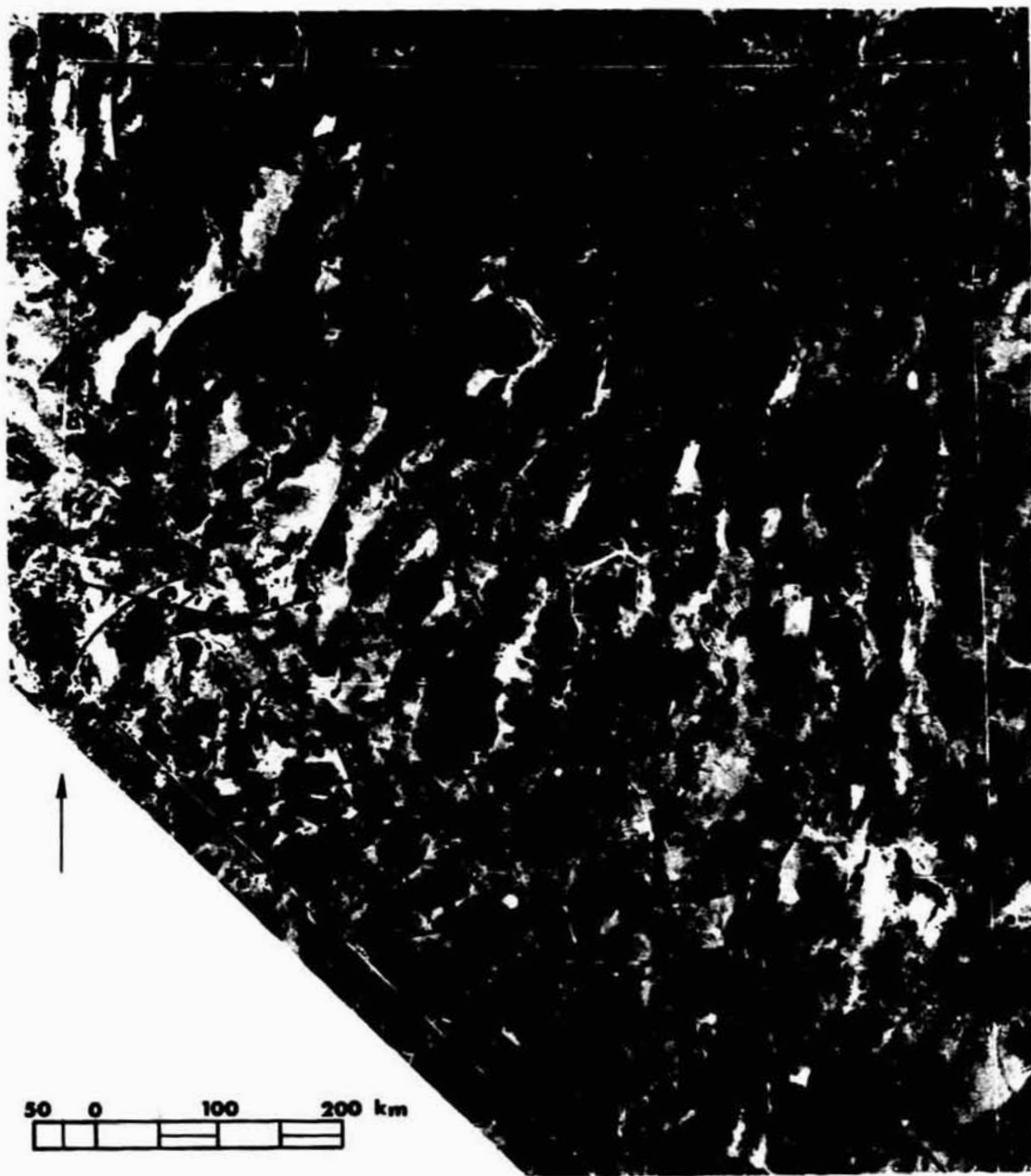
Fig. 1 - ERTS-I mosaic of MSS-5 images obtained in Sept. 1972 showing major lineaments in Nevada, the study area; dashed line shows eastern limit of the area. (Mosaic prepared by Aerial Photographers of Nevada for the University of Nevada, Reno.)
