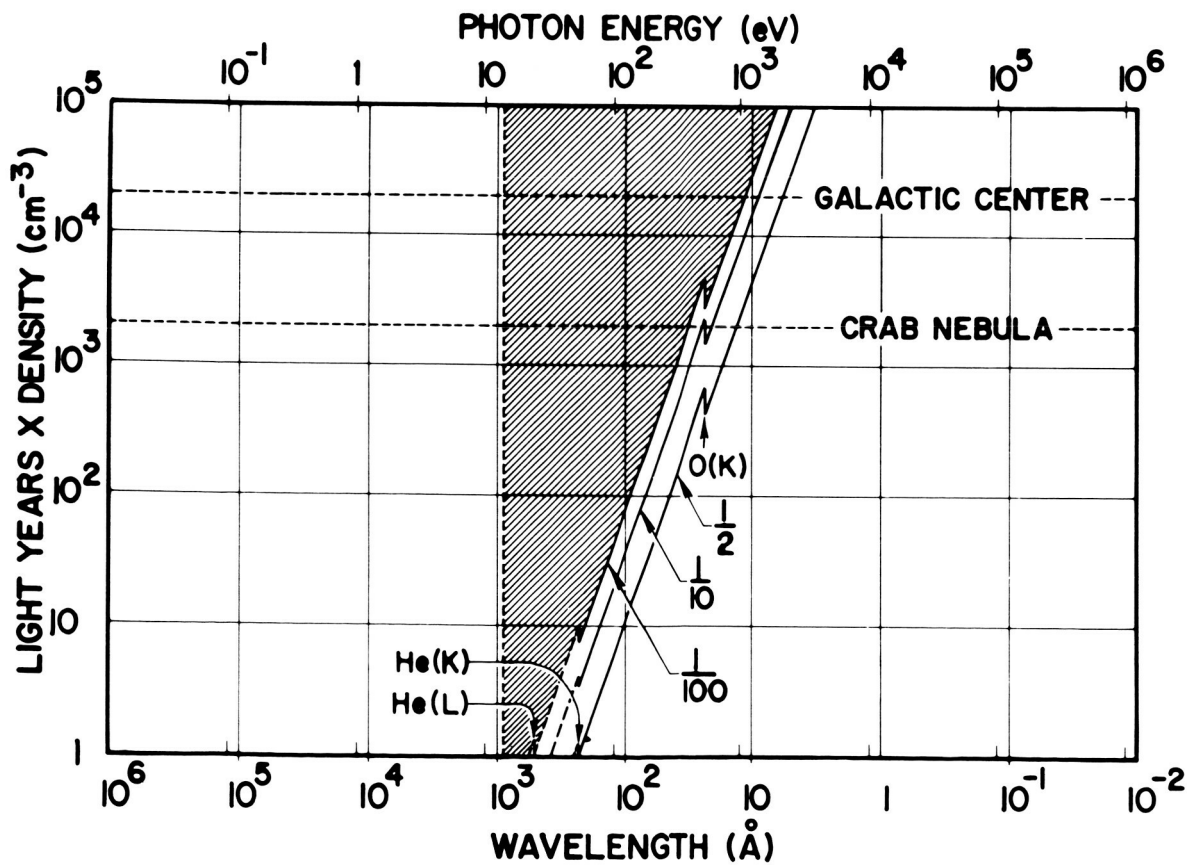
Figure 2. Attenuation of radiation in interstellar space.
