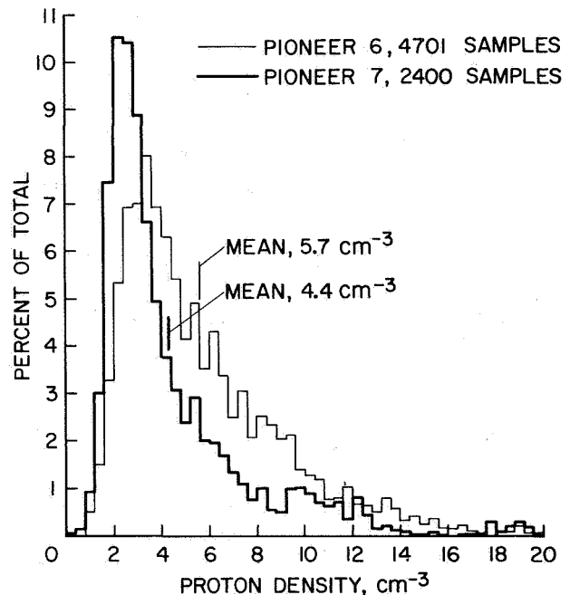
Figure 24. Pioneer 6 and Pioneer 7 proton density histogram.
