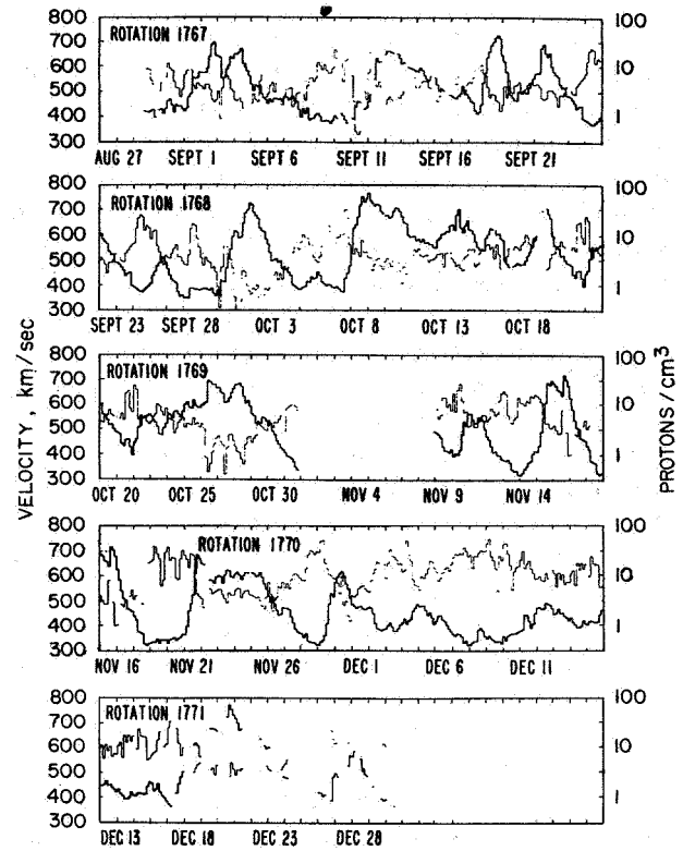
Figure 2. Mariner 2 3-hr average values of plasma velocity and proton number density versus time.
