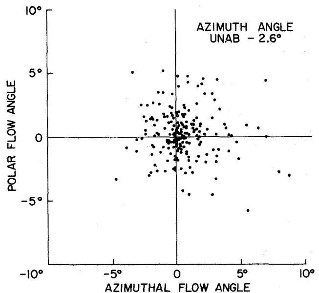
Figure 43. Pioneer 6 polar flow angle as a function of azimuthal flow angle.
