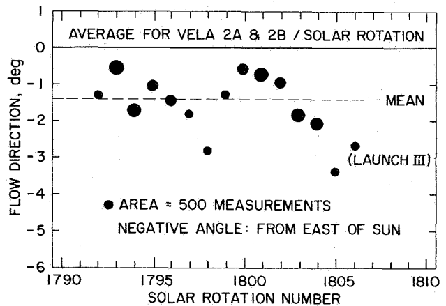
Figure 14. Solar wind flow directions averaged over solar rotations as measured by the Vela 2 satellites from July 1964 to July 1965.
