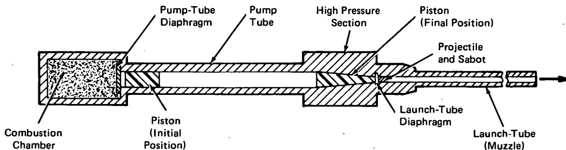
Figure 1. Light-Gas Gun
