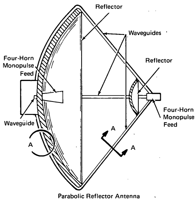
Parabolic Reflector Antenna
