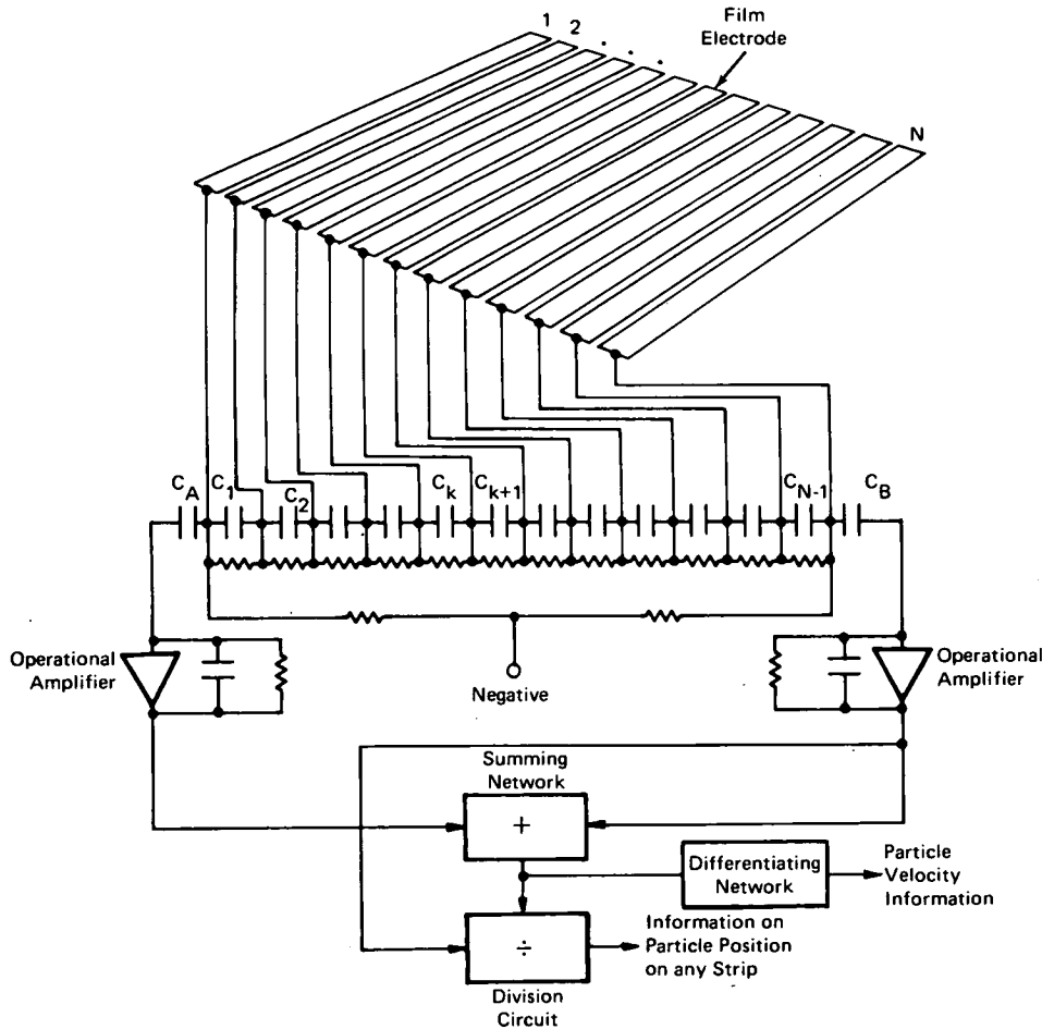
Figure 2. Particle Detector Circuit
