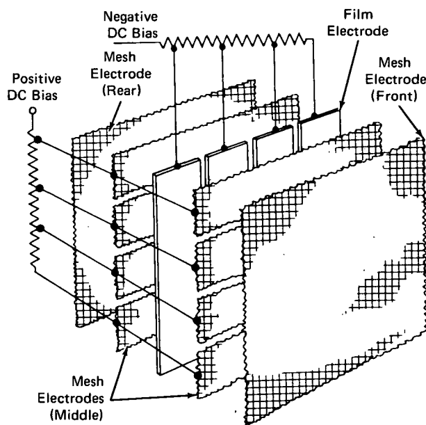
Figure 1. Particle Detector Showing the Five Planar Electrodes
