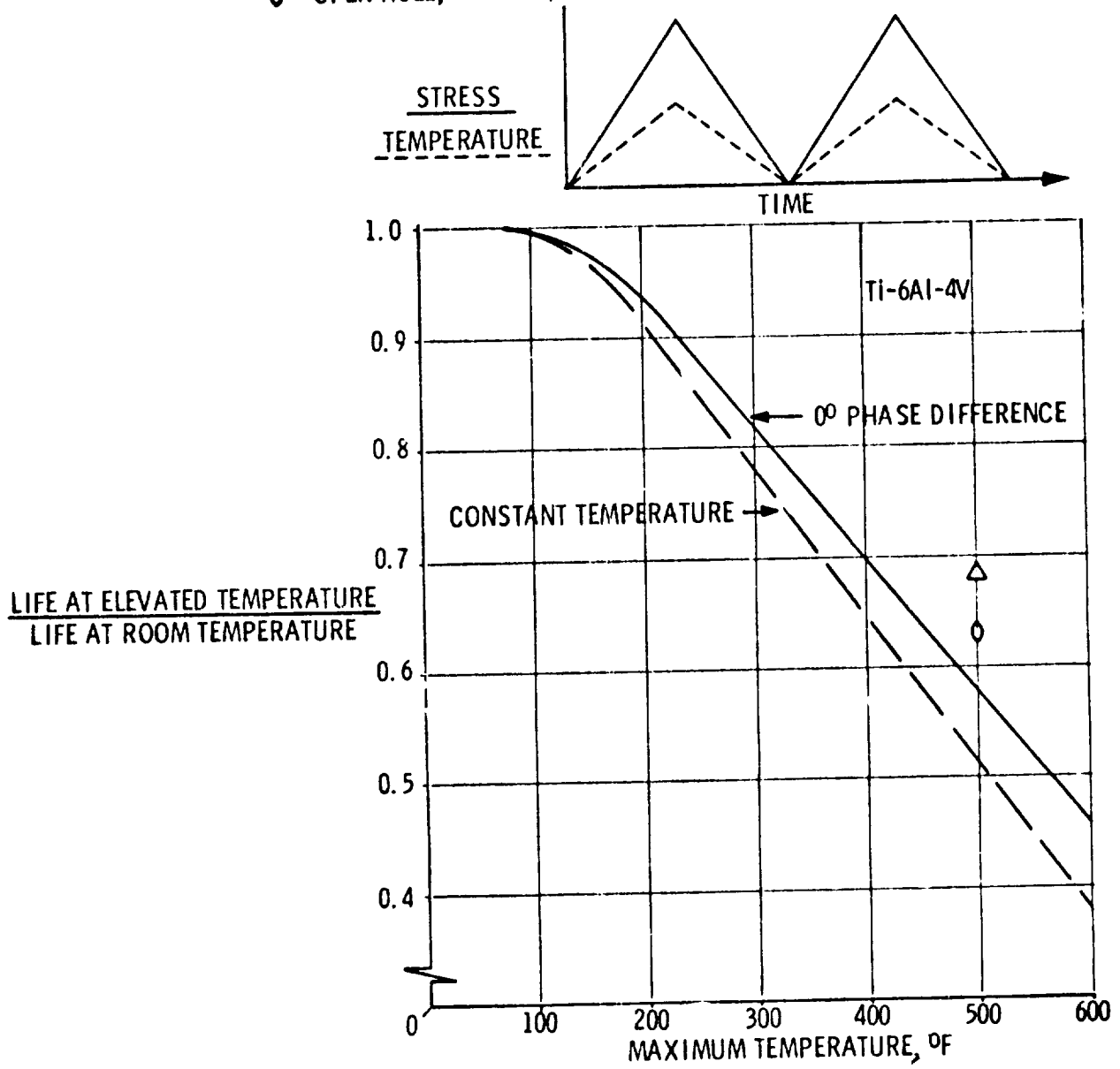
Figure 15.- Life at stress-temperature phase angle of 0°.
