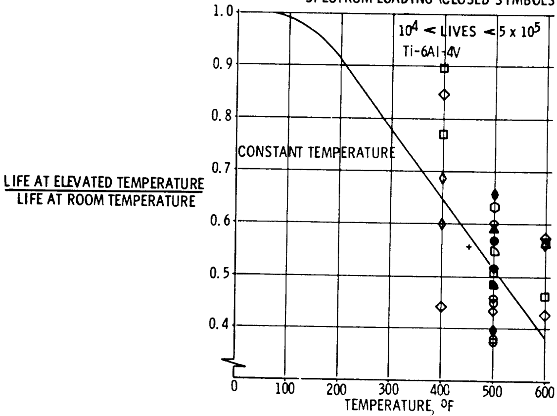
Figure 14.- Life at constant elevated temperature.
