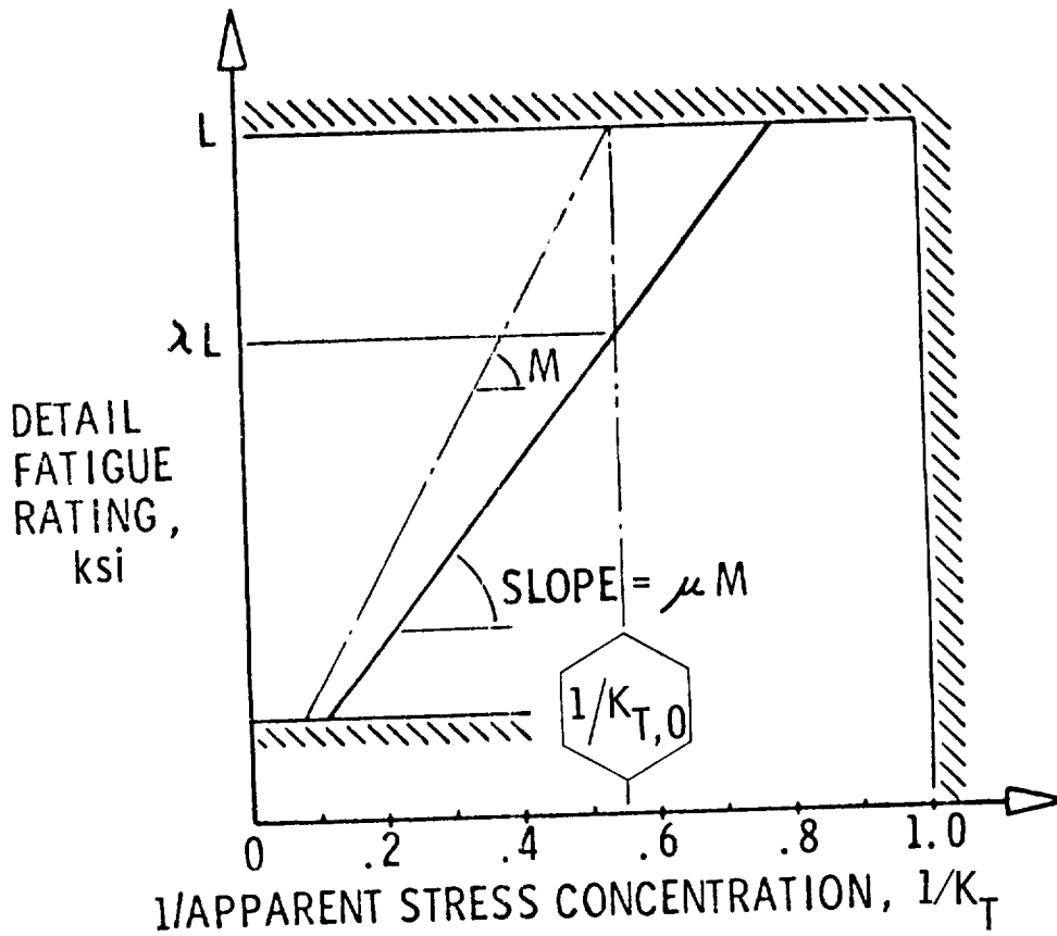
Figure 21.- Detail-fatigue-rating formulation.
