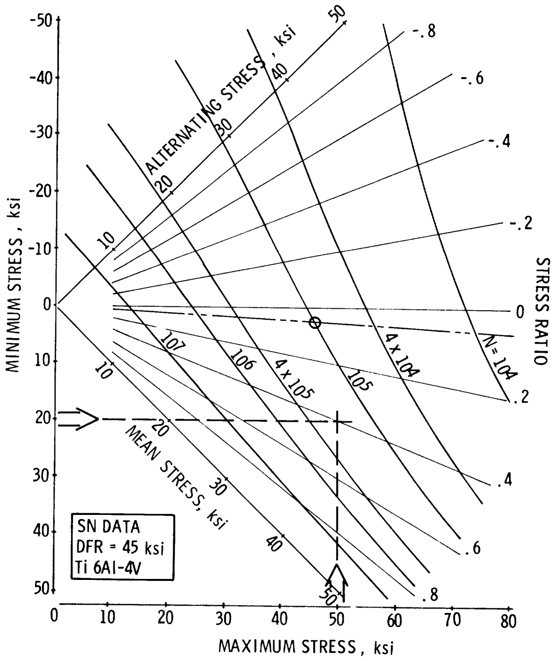
Figure 24.- Constant-life diagram for a component with DFR = 45 ksi.
