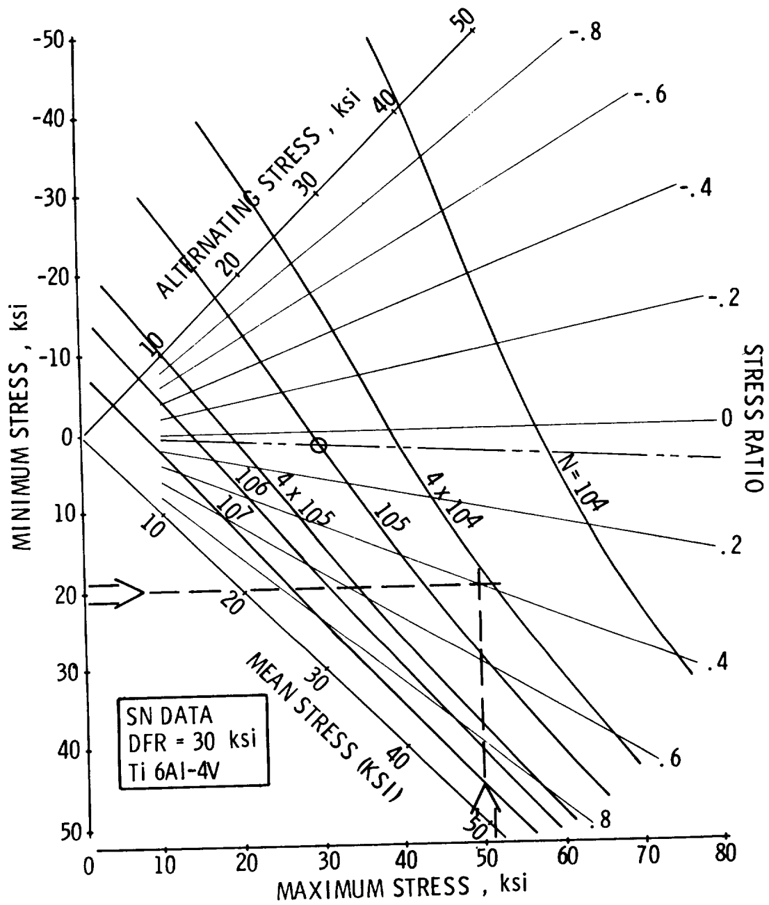
Figure 23.- Constant-life diagram for a component with DFR = 30 ksi.
