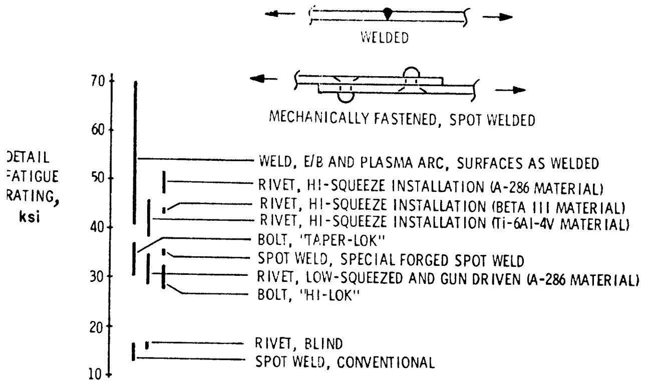
Figure 20.- Ti-6Al-4V joint detail fatigue rating. \sigma_{MAX} at R = 0.06 at 10^5 cycles life.
