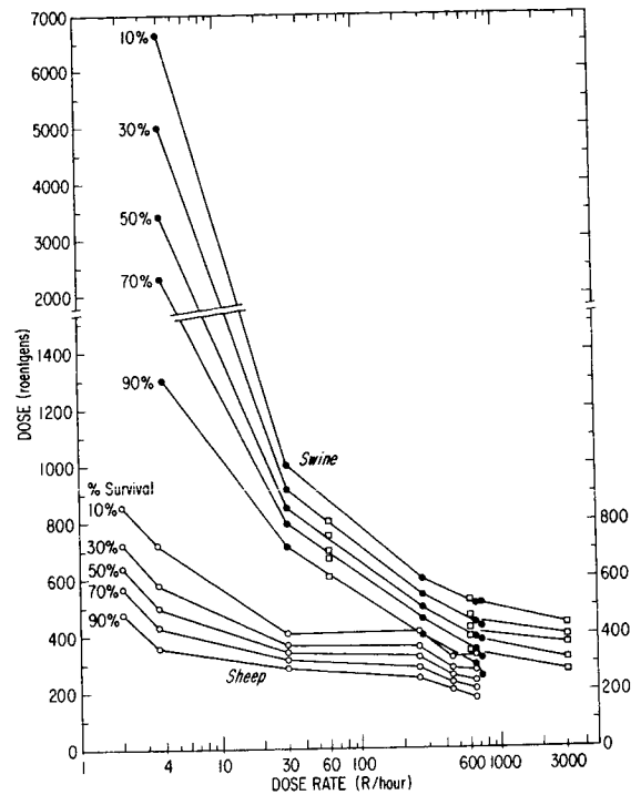
Figure 5. Percent effect dose as related to dose-rate of the exposure.
