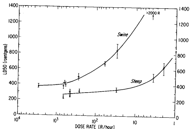
Figure 3. Comparison of radioactivity (LD50) of sheep and swine as related to dose-rate.
