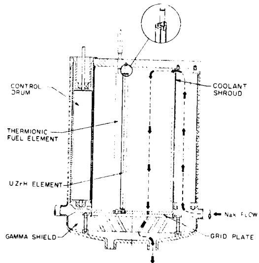
Fig. 6. Reactor Elevation Cross Section
