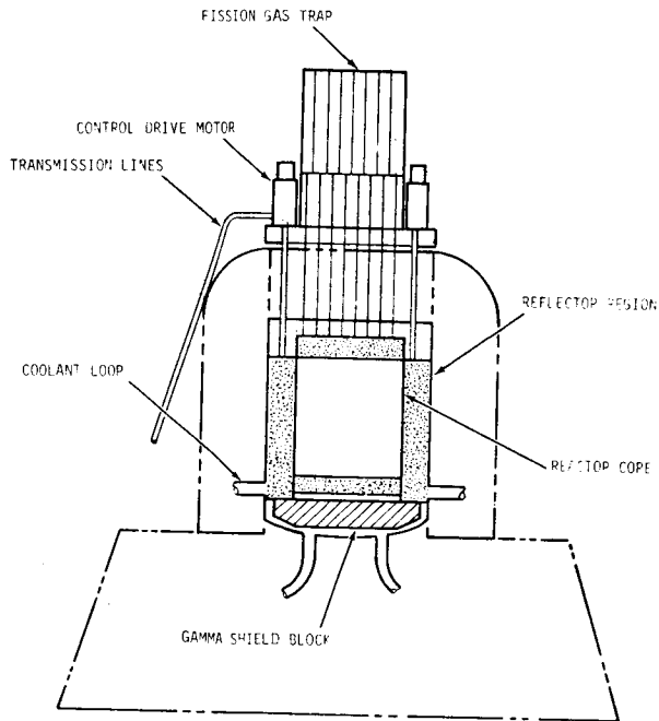
Fig. 4. Reactor Subassembly
