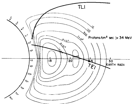
GEOMAGNETIC TRAJECTORIES OF TRANSLUNAR AND TRANS-EARTH INJECTION OF APOLLO XII MISSION Figure 1
