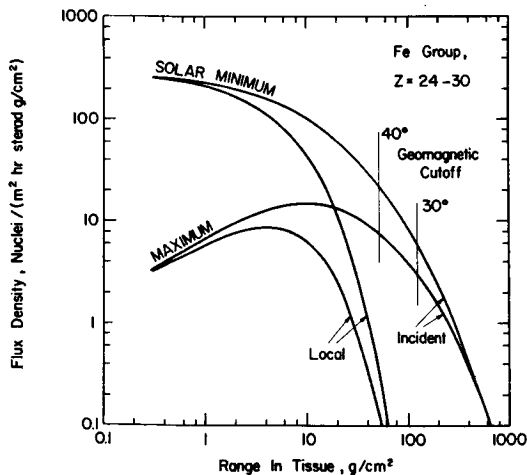
DIFFERENTIAL RANGE SPECTRA FOR IRON GROUP AT SOLAR MAXIMUM AND MINIMUM
