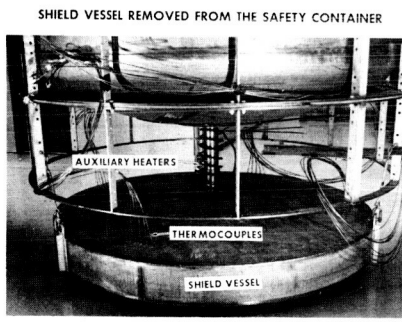
Figure 5.--Shield Vessel Removed from the Safety Container
