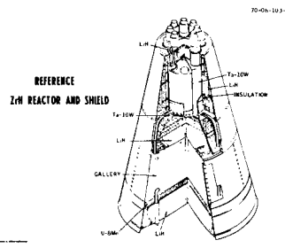
Figure 1.—Reference ZrH Reactor and Shield
