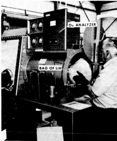
LOADING BAGS OF LiH INTO THE DRY BOX ANTECHAMBER
