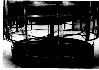
Figure 14.—Cast LiH Shield Lifted from the Safety Container
