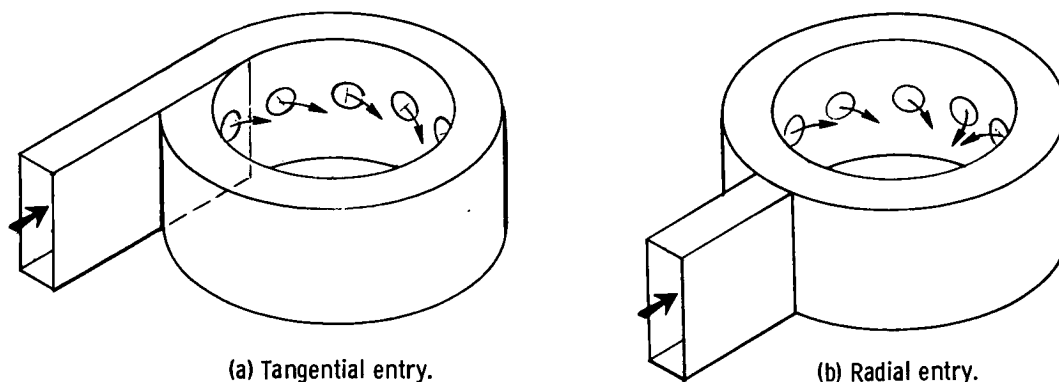
Circumferential manifold.
