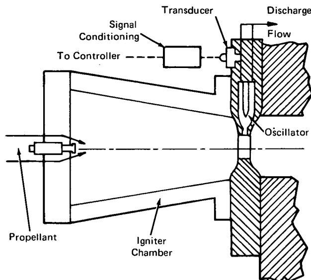
Ignition Sensor Assembly Schematic Figure 2.
