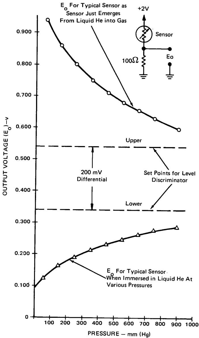
Figure 2. Operational characteristics of the level detector and indicator system.
